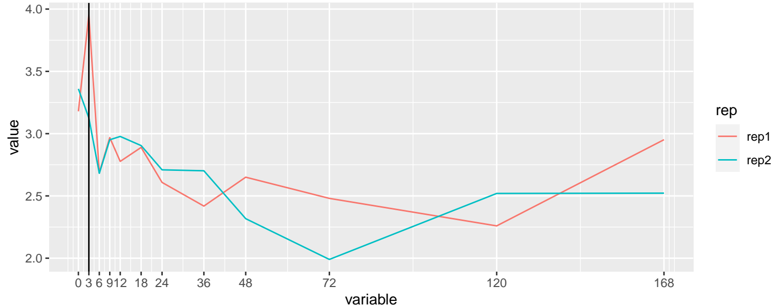
Regression: ENSG00000088179 – H3K4me1
