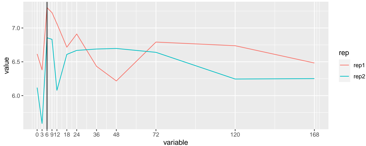
Regression: ENSG00000157827 – H3K4me1
