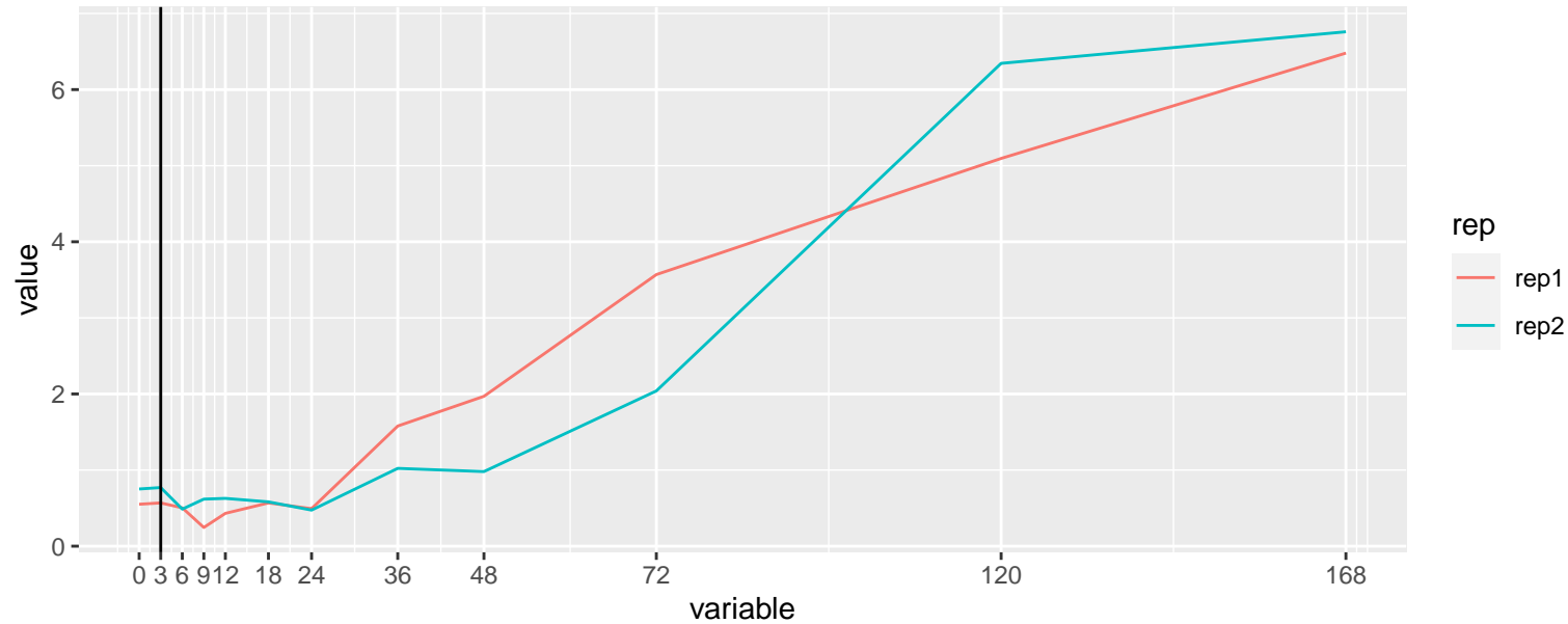
Regression: ENSG00000136250 – H3K4me1
