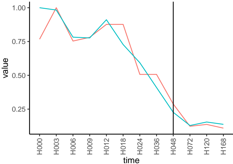
Normalized signals – ENSG00000114631 pre-not-downregulated/post-not-downregula
