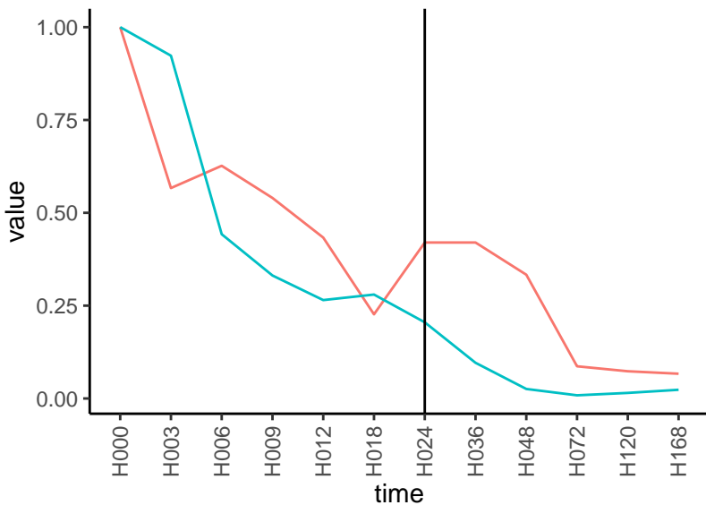
Normalized signals – ENSG00000133067 pre-not-downregulated/post-downregulated
