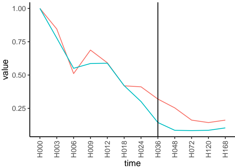
Normalized signals – ENSG00000184185 pre-not-downregulated/post-not-downregula
