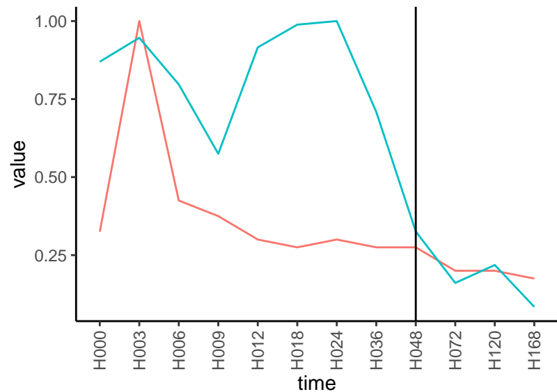
Normalized signals – ENSG00000101188 pre-not-downregulated/post-not-downregula
