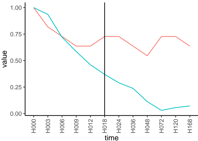
Normalized signals – ENSG00000172264 pre-not-downregulated/post-not-downregula
