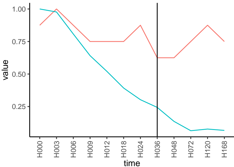
Normalized signals – ENSG00000152611 pre-not-downregulated/post-not-downregula
