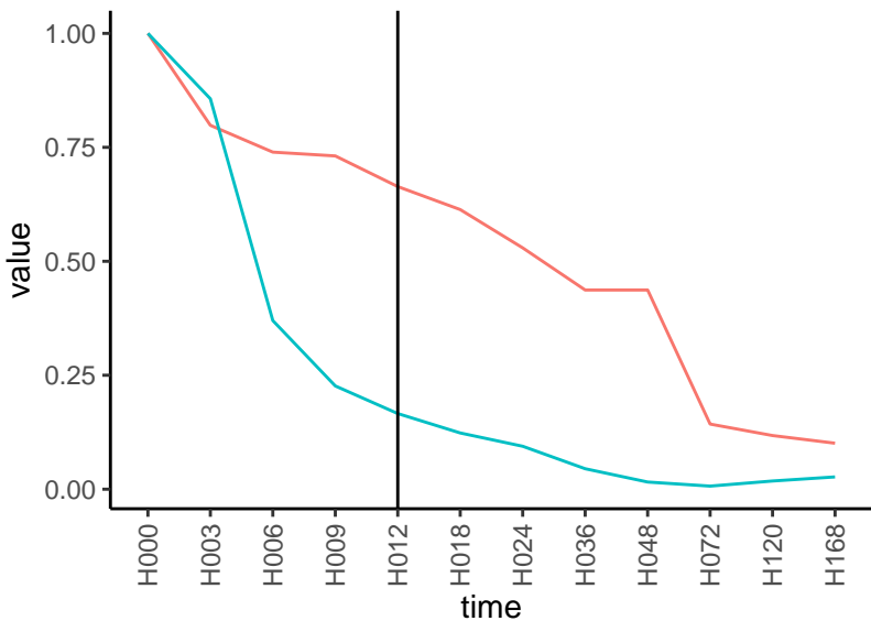
Normalized signals – ENSG00000077943 pre-not-downregulated/post-not-downregula
