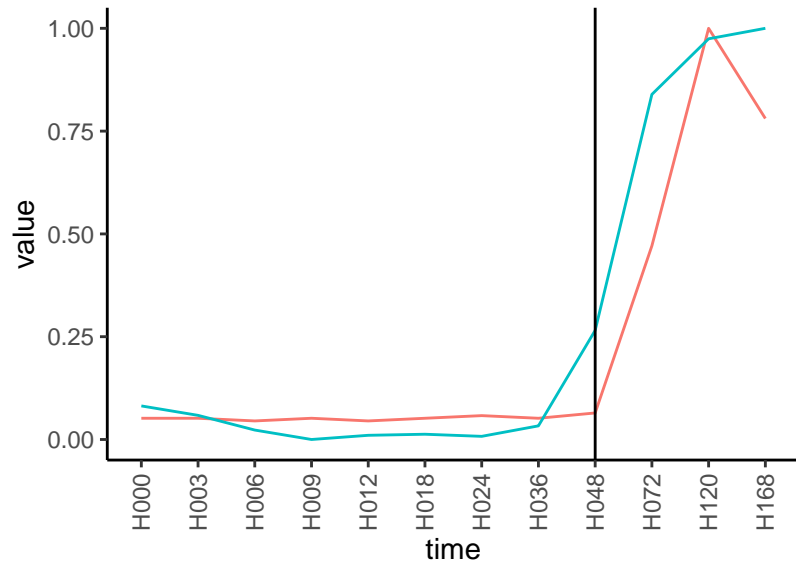
Normalized signals – ENSG00000121594 pre-not-upregulated/post-upregulated
