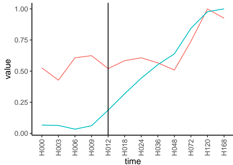
Normalized signals – ENSG00000011600 pre-not-upregulated/post-upregulated
