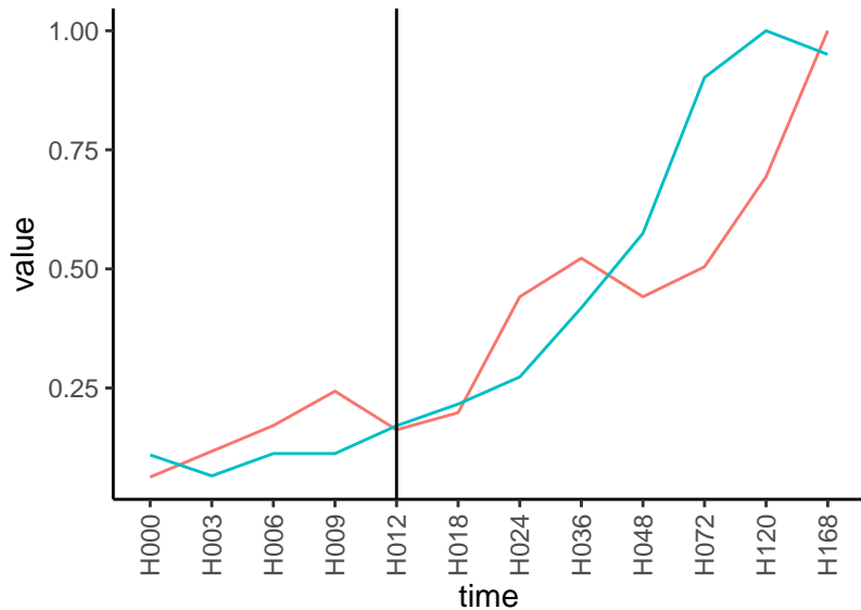
Normalized signals – ENSG00000244482 pre-not-upregulated/post-upregulated
