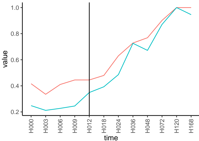
Normalized signals – ENSG00000177191 pre-not-upregulated/post-upregulated
