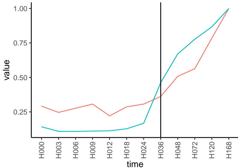
Normalized signals – ENSG00000116574 pre-not-upregulated/post-upregulated
