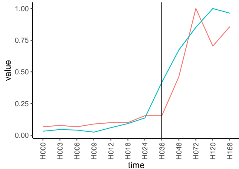
Normalized signals – ENSG00000172322 pre-not-upregulated/post-upregulated
