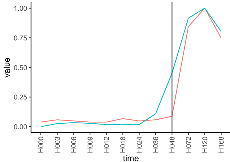
Normalized signals – ENSG00000147883 pre-not-upregulated/post-not-upregulated
