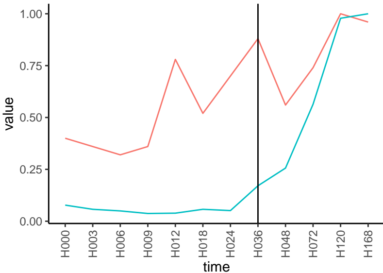
Normalized signals – ENSG00000104921 pre-not-upregulated/post-not-upregulated
