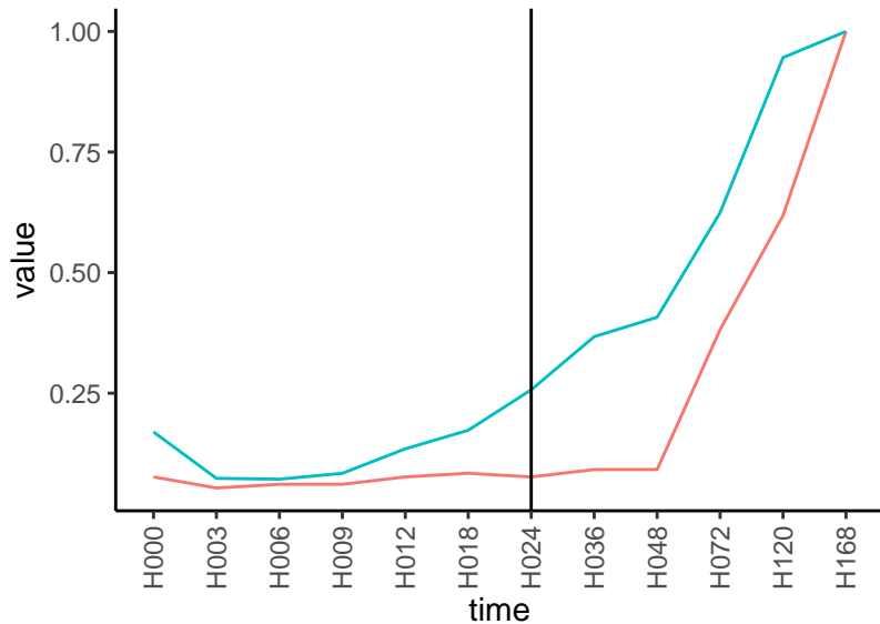
Normalized signals – ENSG00000133574 pre-not-upregulated/post-upregulated
