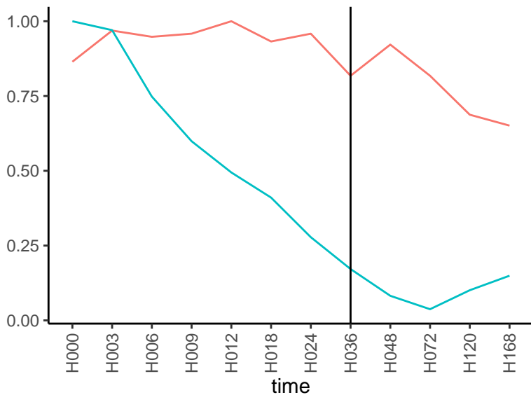
Normalized signals – ENSG00000165078 pre-not-downregulated/post-downregulated
