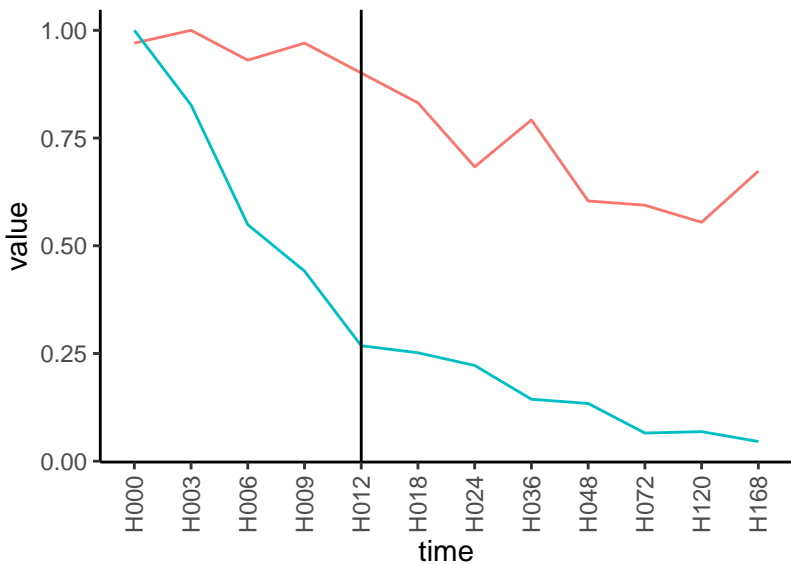
Normalized signals – ENSG00000157087 pre-not-downregulated/post-not-downregula
