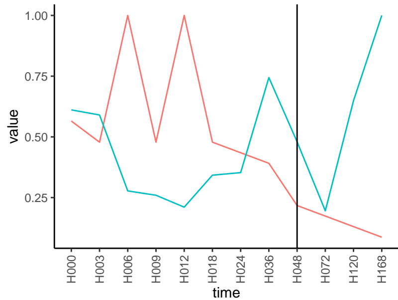
Normalized signals – ENSG00000232653
