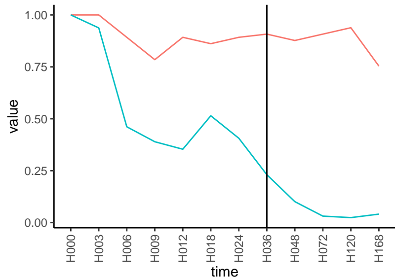
Normalized signals – ENSG00000128833 pre-not-downregulated/post-not-downregula
