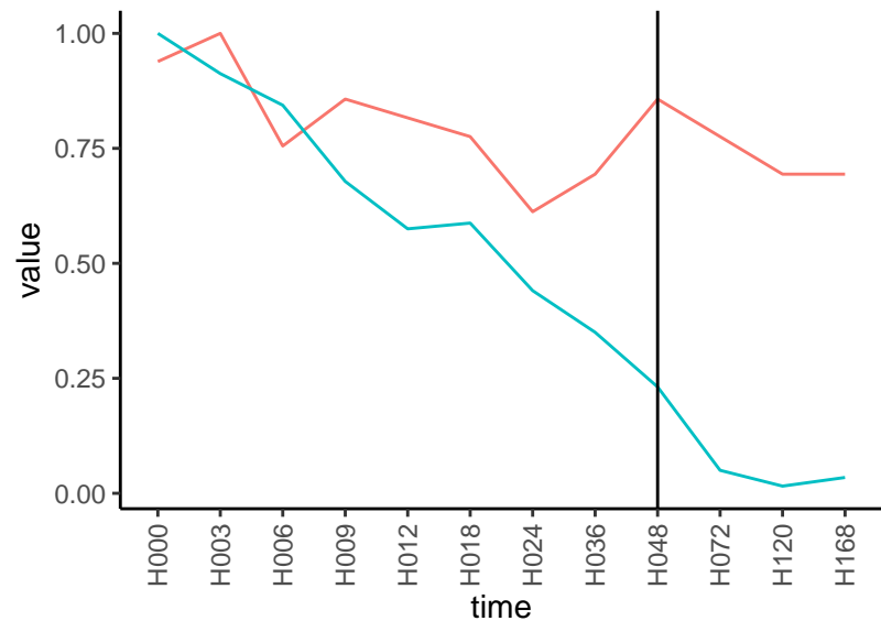
Normalized signals – ENSG00000166402 pre-not-downregulated/post-not-downregula
