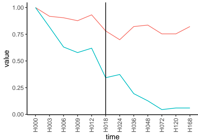
Normalized signals – ENSG00000152969 pre-not-downregulated/post-not-downregula
