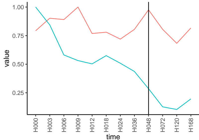
Normalized signals – ENSG00000151692 pre-not-downregulated/post-not-downregula
