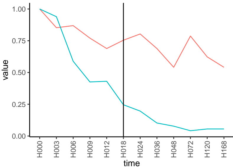
Normalized signals – ENSG00000100290 pre-not-downregulated/post-downregulated
