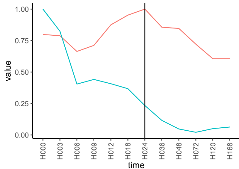
Normalized signals – ENSG00000178217 pre-not-downregulated/post-downregulated
