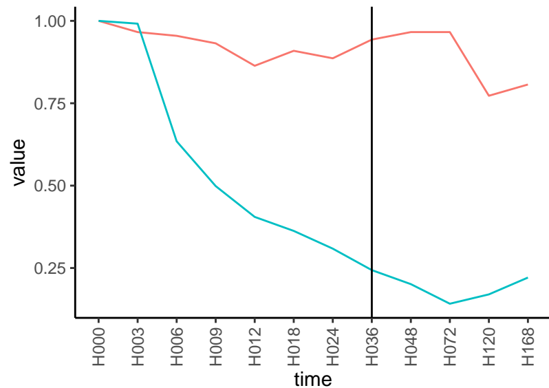
Normalized signals – ENSG00000090975 pre-not-downregulated/post-downregulated
