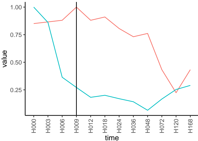
Normalized signals – ENSG00000172575 pre-not-downregulated/post-downregulated
