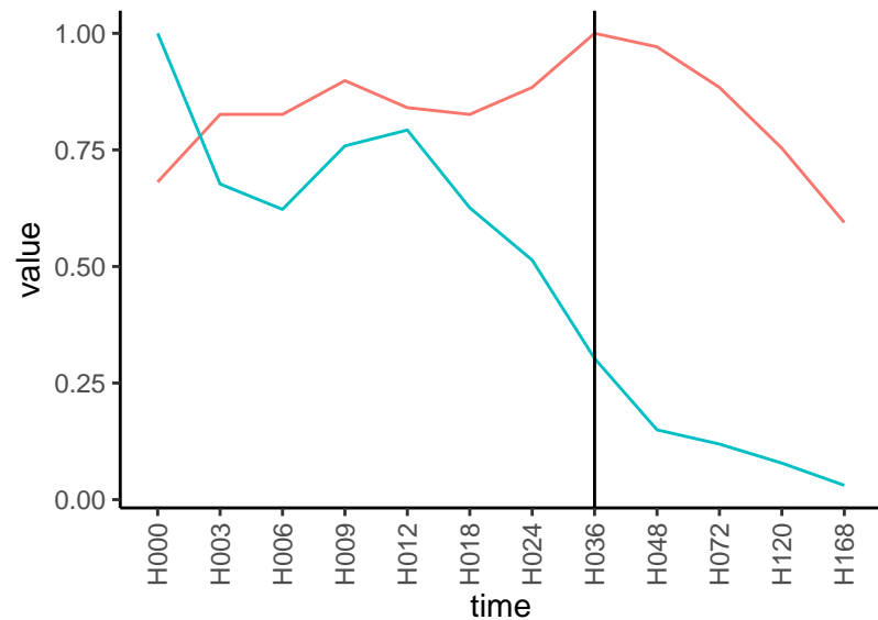
Normalized signals – ENSG00000145911 pre-not-downregulated/post-downregulated
