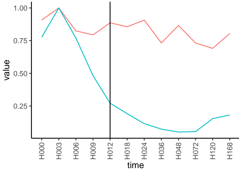
Normalized signals – ENSG00000146592 pre-not-downregulated/post-downregulated
