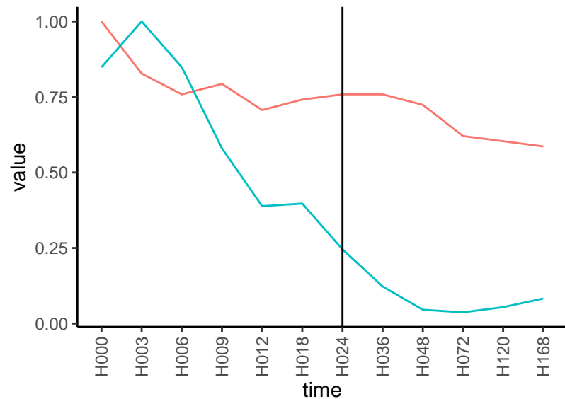
Normalized signals – ENSG00000136237 pre-not-downregulated/post-downregulated
