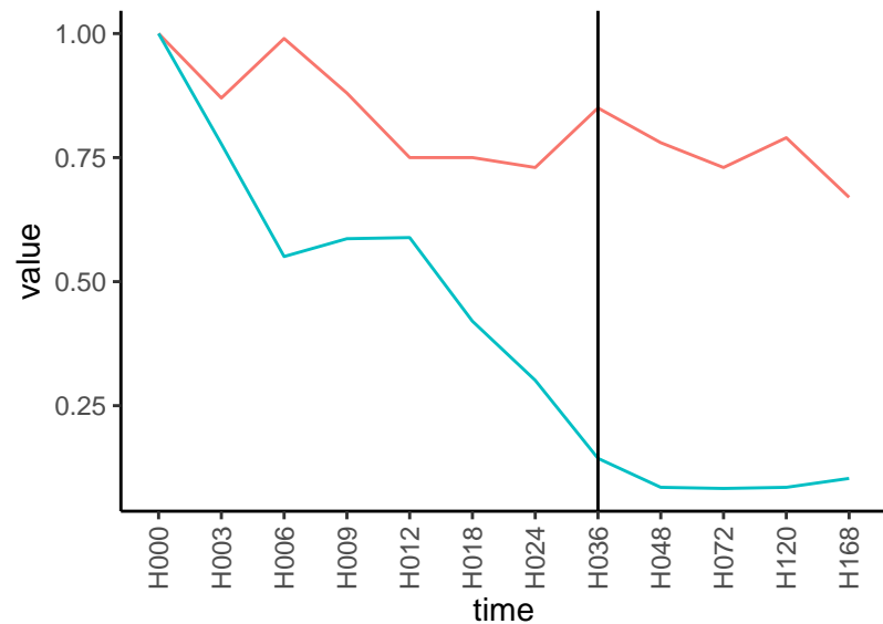
Normalized signals – ENSG00000184185 pre-not-downregulated/post-not-downregula
