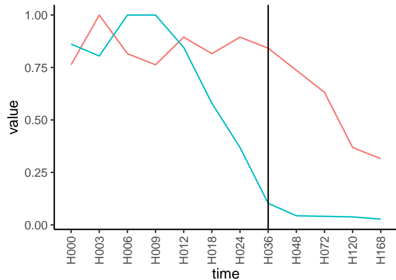
Normalized signals – ENSG00000137693 pre-not-downregulated/post-downregulated
