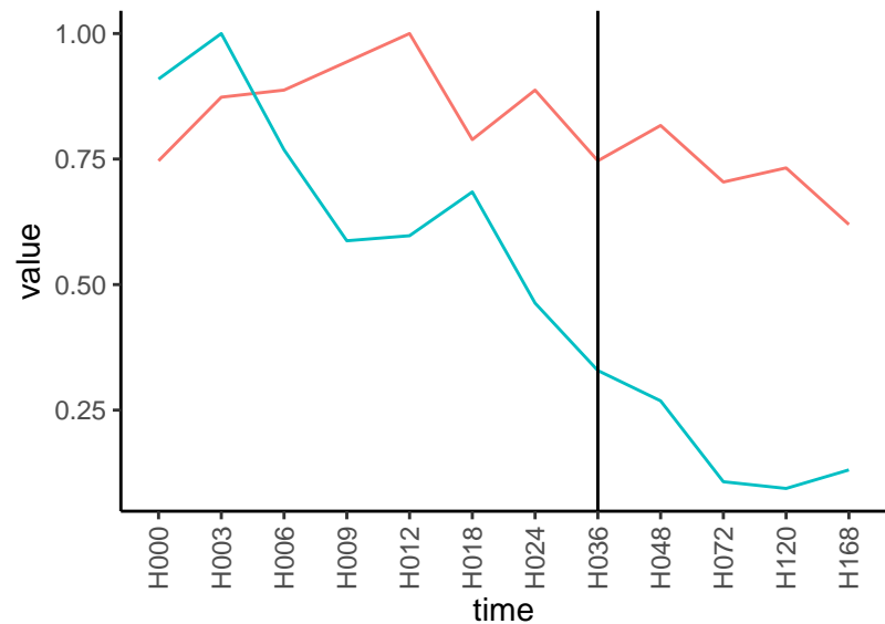
Normalized signals – ENSG00000140557 pre-not-downregulated/post-not-downregula
