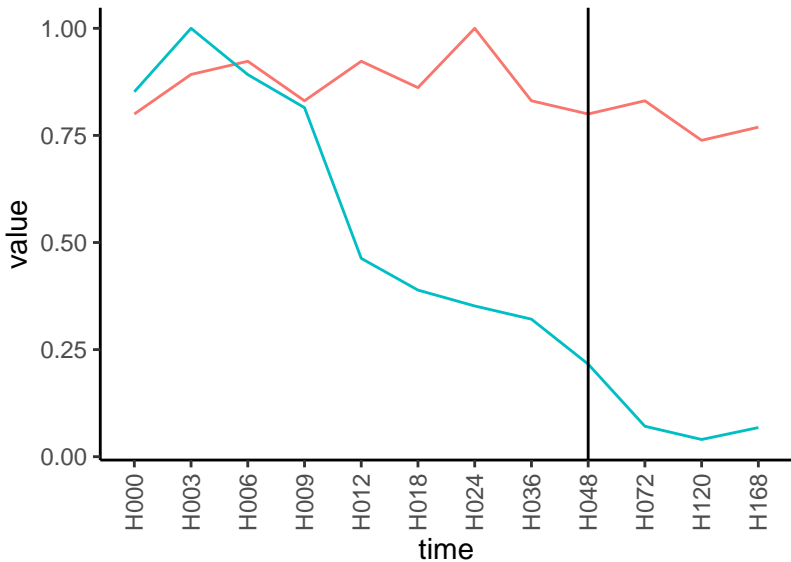
Normalized signals – ENSG00000182621 pre-not-downregulated/post-not-downregula
