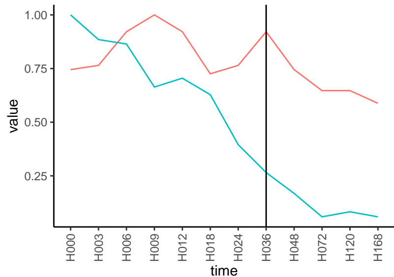
Normalized signals – ENSG00000182272 pre-not-downregulated/post-not-downregula
