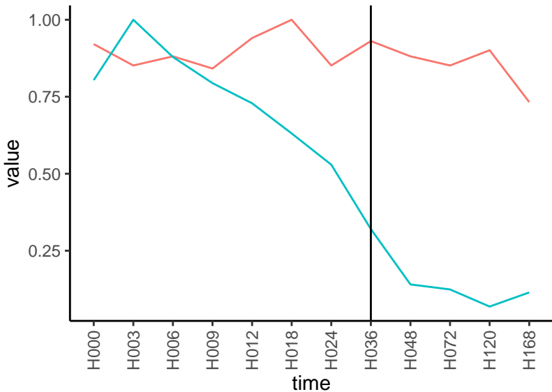
Normalized signals – ENSG00000078269 pre-not-downregulated/post-not-downregula
