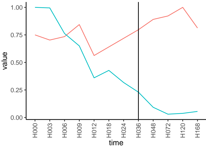
Normalized signals – ENSG00000145934 pre-not-downregulated/post-not-downregula
