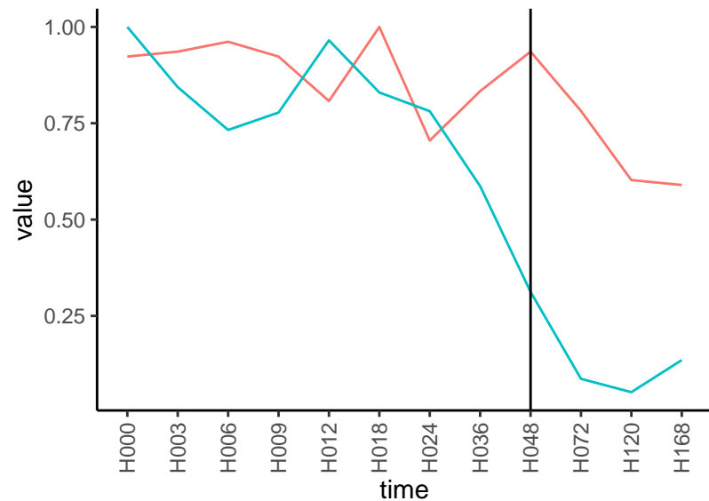
Normalized signals – ENSG00000173805 pre-not-downregulated/post-downregulated
