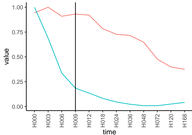
Normalized signals – ENSG00000136883 pre-not-downregulated/post-downregulated
