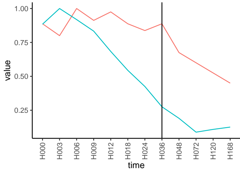
Normalized signals – ENSG00000176749 pre-not-downregulated/post-not-downregula
