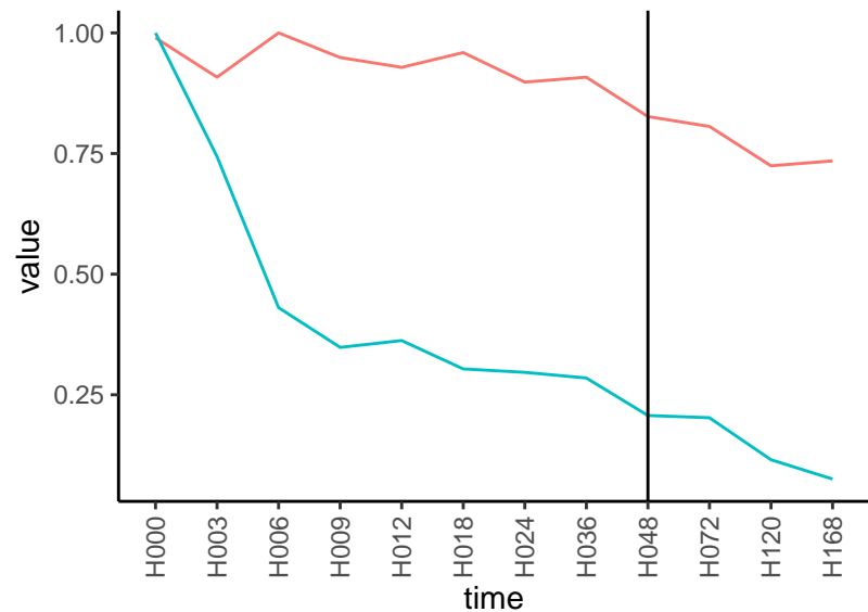
Normalized signals – ENSG00000092758 pre-not-downregulated/post-not-downregula
