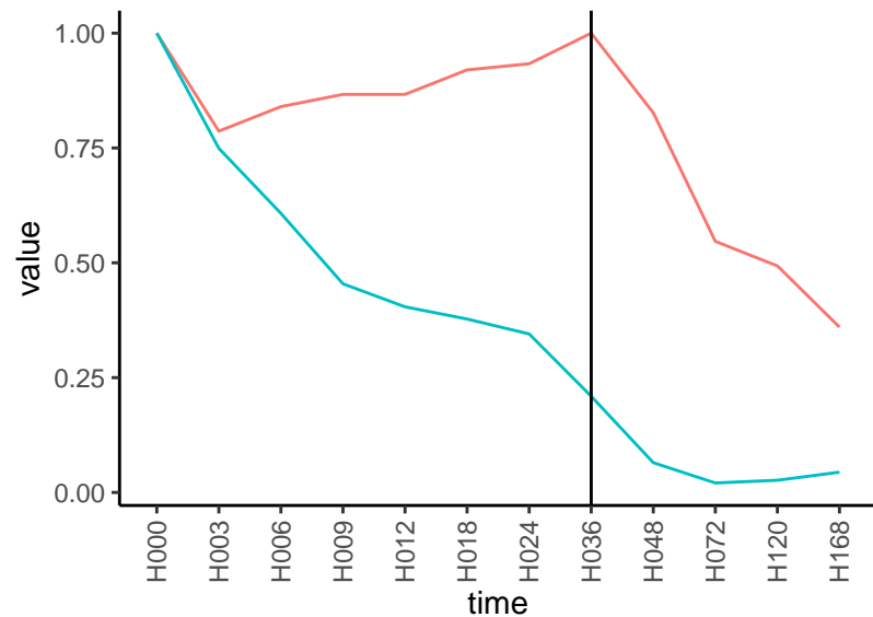
Normalized signals – ENSG00000215045 pre-not-downregulated/post-downregulated
