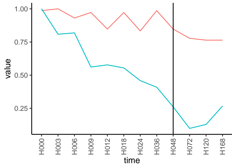
Normalized signals – ENSG00000099958 pre-not-downregulated/post-not-downregula
