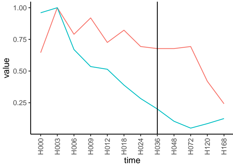
Normalized signals – ENSG00000185737 pre-not-downregulated/post-downregulated
