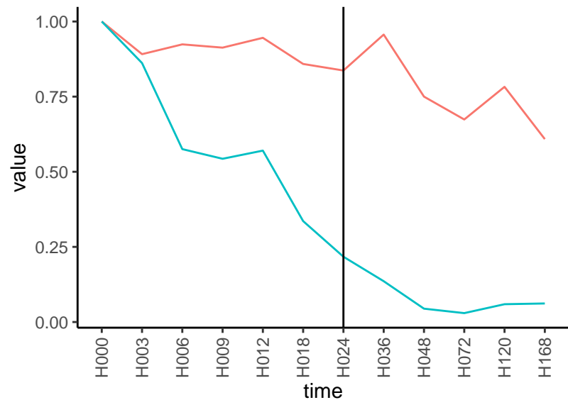
Normalized signals – ENSG00000187922 pre-not-downregulated/post-not-downregula
