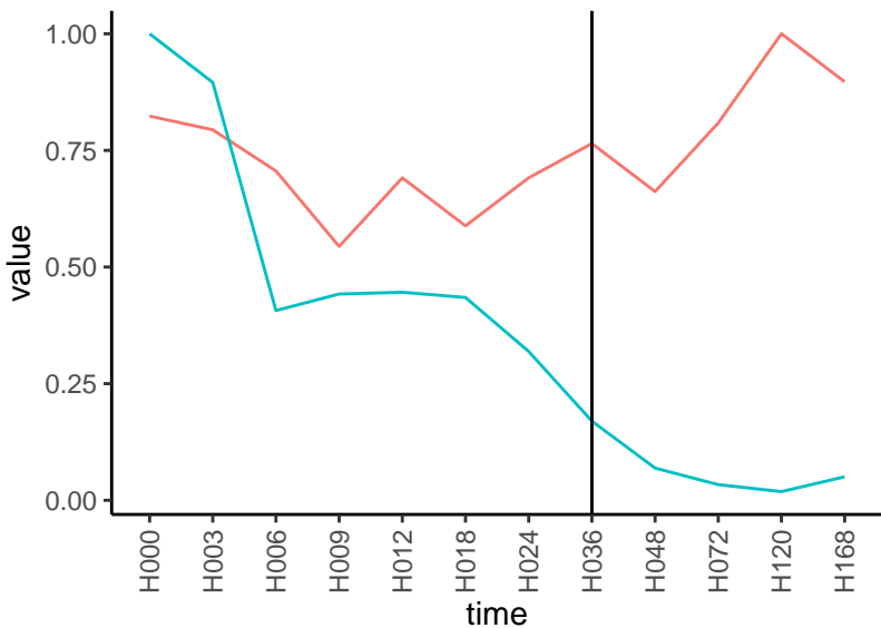
Normalized signals – ENSG00000172995 pre-not-downregulated/post-not-downregula
