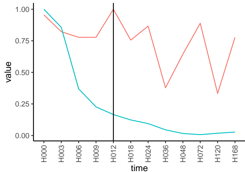
Normalized signals – ENSG00000077943 pre-not-downregulated/post-not-downregula
