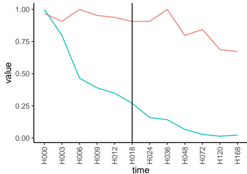
Normalized signals – ENSG00000165905 pre-not-downregulated/post-downregulated
