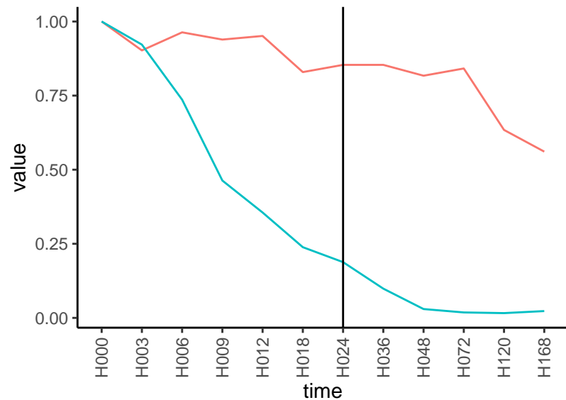
Normalized signals – ENSG00000015413 pre-not-downregulated/post-downregulated
