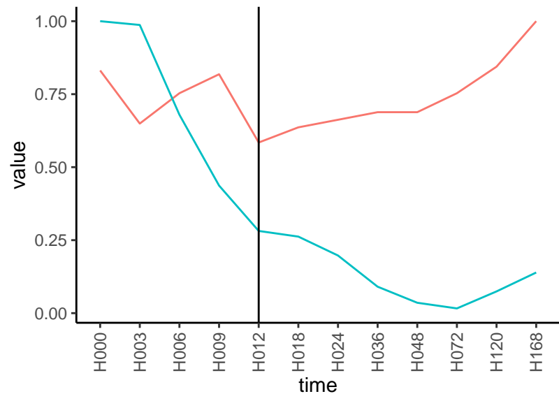
Normalized signals – ENSG00000149256 pre-not-downregulated/post-not-downregula
