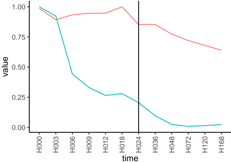
Normalized signals – ENSG00000133067 pre-not-downregulated/post-not-downregula
