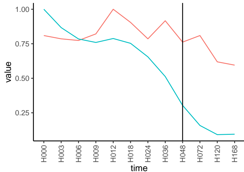
Normalized signals – ENSG00000001617 pre-not-downregulated/post-downregulated
