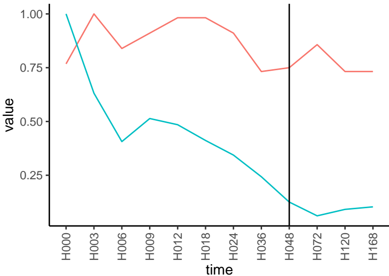
Normalized signals – ENSG00000175097 pre-not-downregulated/post-not-downregula
