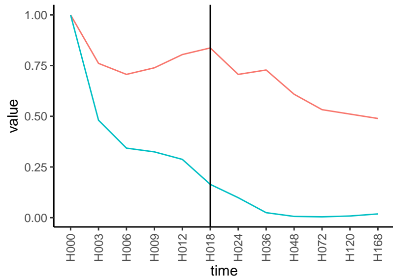
Normalized signals – ENSG00000185028 pre-not-downregulated/post-downregulated
