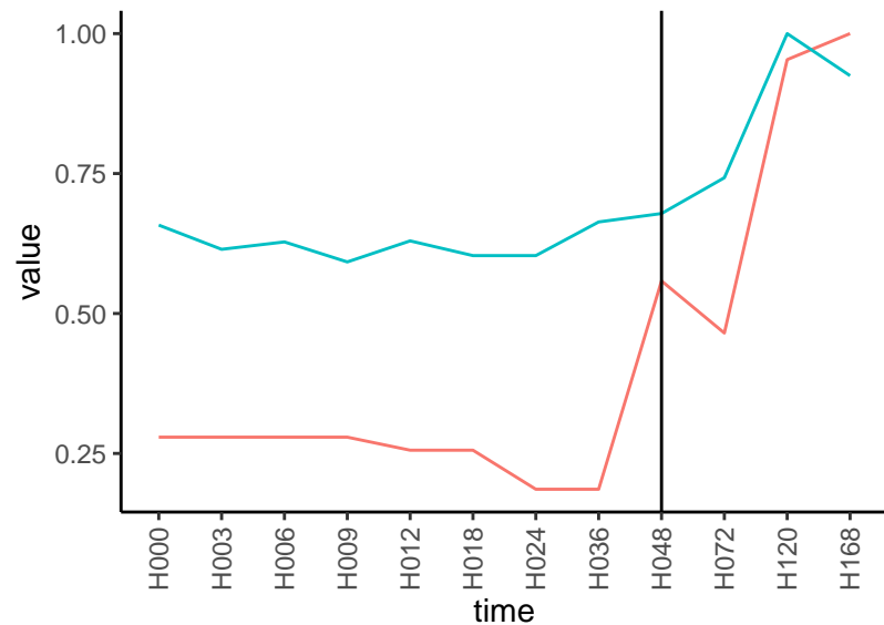
Normalized signals – ENSG00000167702 pre-not-upregulated/post-not-upregulated
