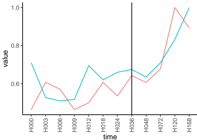
Normalized signals – ENSG00000169964 pre-not-upregulated/post-upregulated
