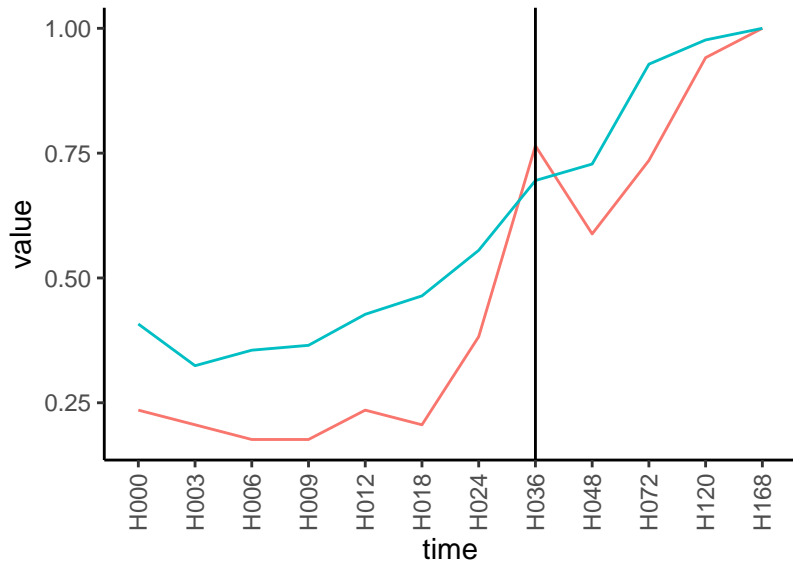
Normalized signals – ENSG00000105711 pre-not-upregulated/post-not-upregulated
