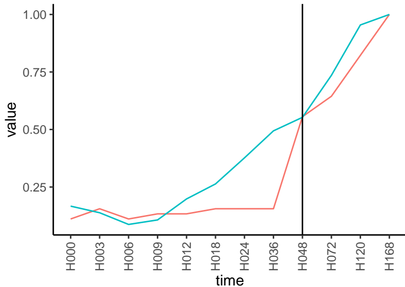
Normalized signals – ENSG00000114013 pre-not-upregulated/post-upregulated
