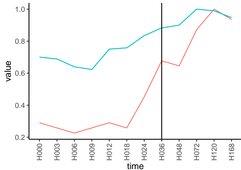
Normalized signals – ENSG00000105048 pre-not-upregulated/post-not-upregulated
