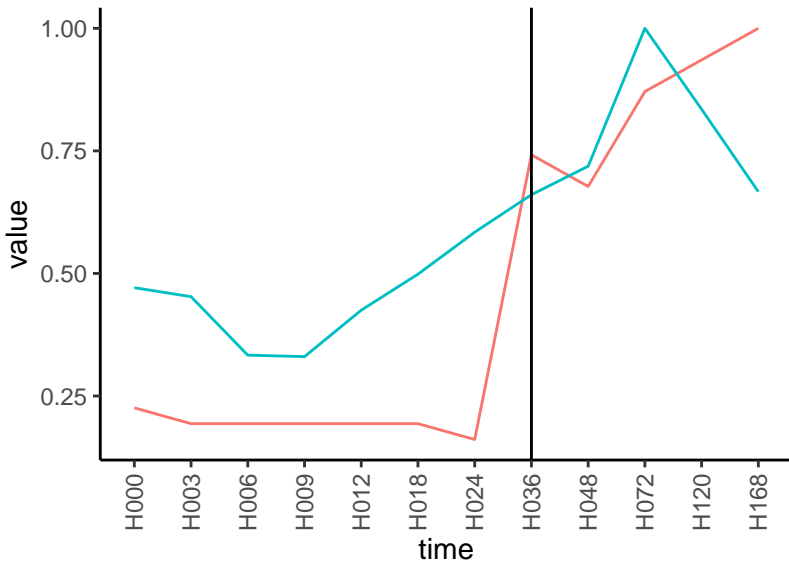
Normalized signals – ENSG00000162390 pre-not-upregulated/post-not-upregulated
