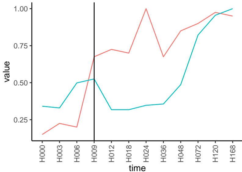
Normalized signals – ENSG00000137449 pre-not-upregulated/post-upregulated
