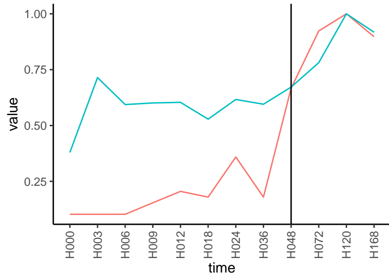
Normalized signals – ENSG00000177606 pre-not-upregulated/post-not-upregulated
