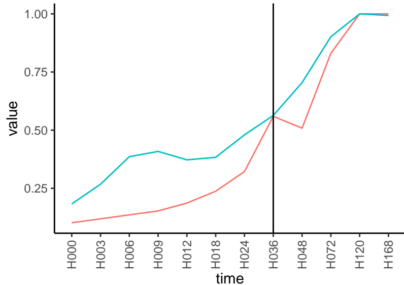
Normalized signals – ENSG00000033627 pre-not-upregulated/post-upregulated
