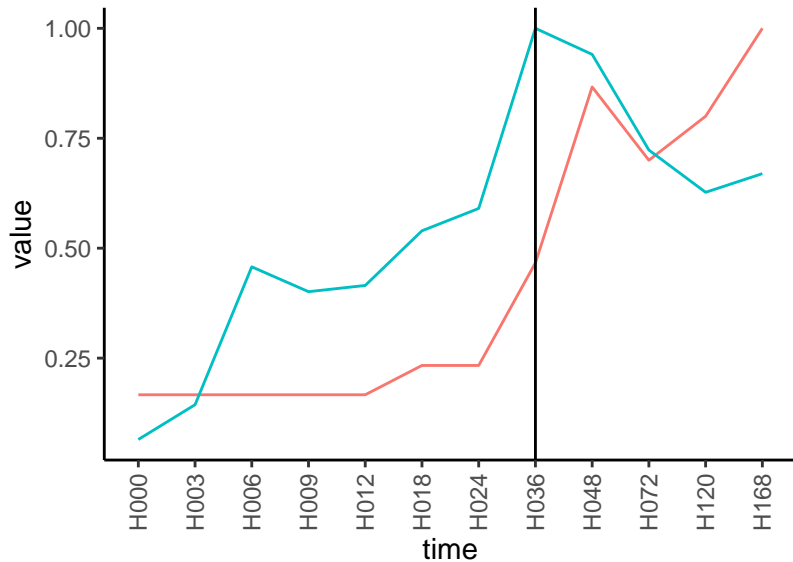
Normalized signals – ENSG00000187912 pre-not-upregulated/post-not-upregulated
