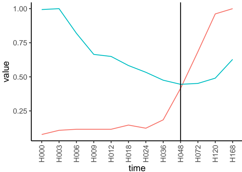
Normalized signals – ENSG00000027075 pre-not-upregulated/post-not-upregulated
