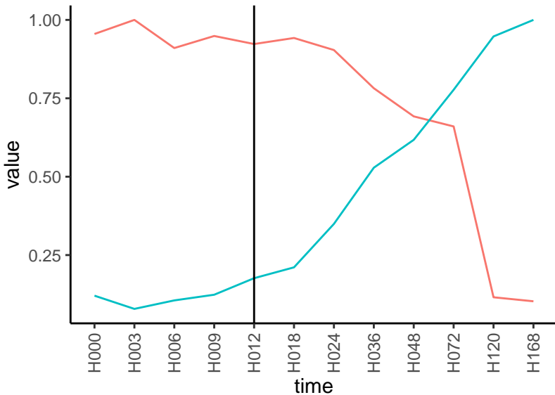
Normalized signals – ENSG00000134955 pre-not-upregulated/post-not-upregulated
