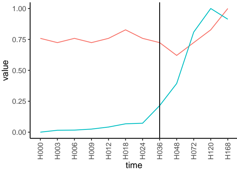
Normalized signals – ENSG00000155659 pre-not-upregulated/post-not-upregulated
