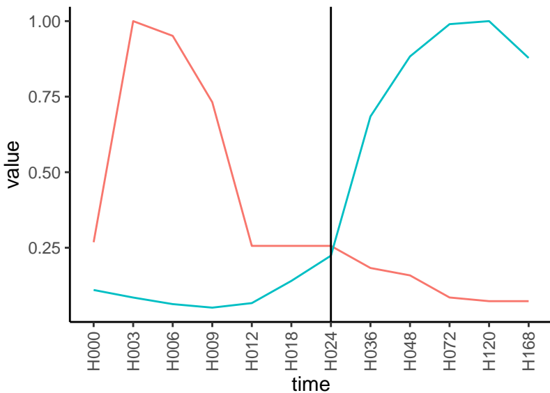
Normalized signals – ENSG00000000938 pre-not-upregulated/post-not-upregulated
