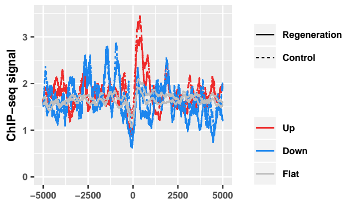
Genic_exonic: H3K3me1 at 0h
