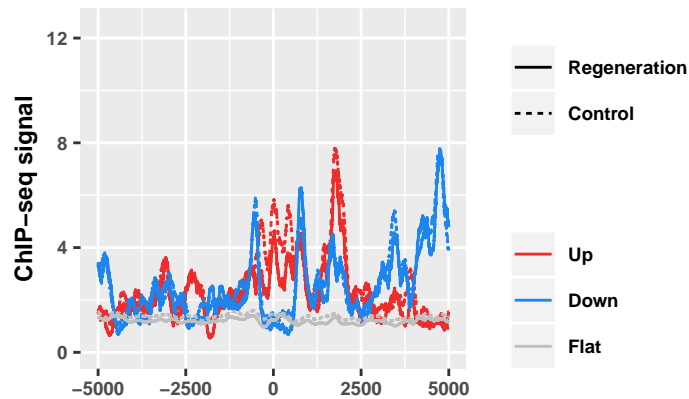
Intergenic: RNAPol-II at 0h
