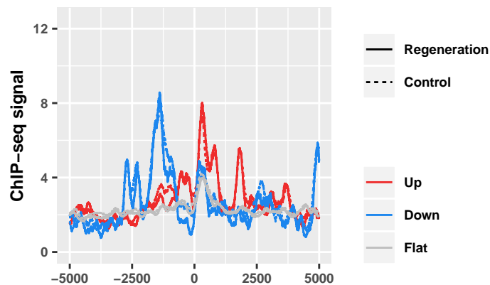
Genic_exonic: RNAPol-II at 0h
