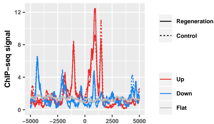
Genic_intronic: RNAPol-II at 0h
