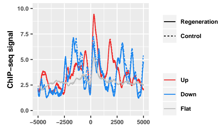
Genic_exonic: H3K27ac at 0h
