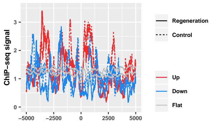
Genic_intronic: H3K3me1 at 0h
