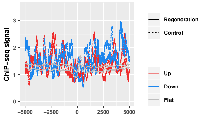
Intergenic: H3K3me1 at 0h
