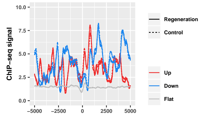
Intergenic: H3K27ac at 0h
