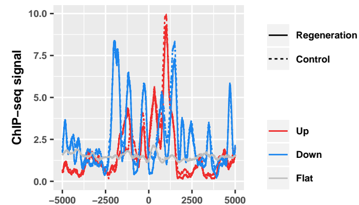
Genic_intronic: H3K27ac at 0h
