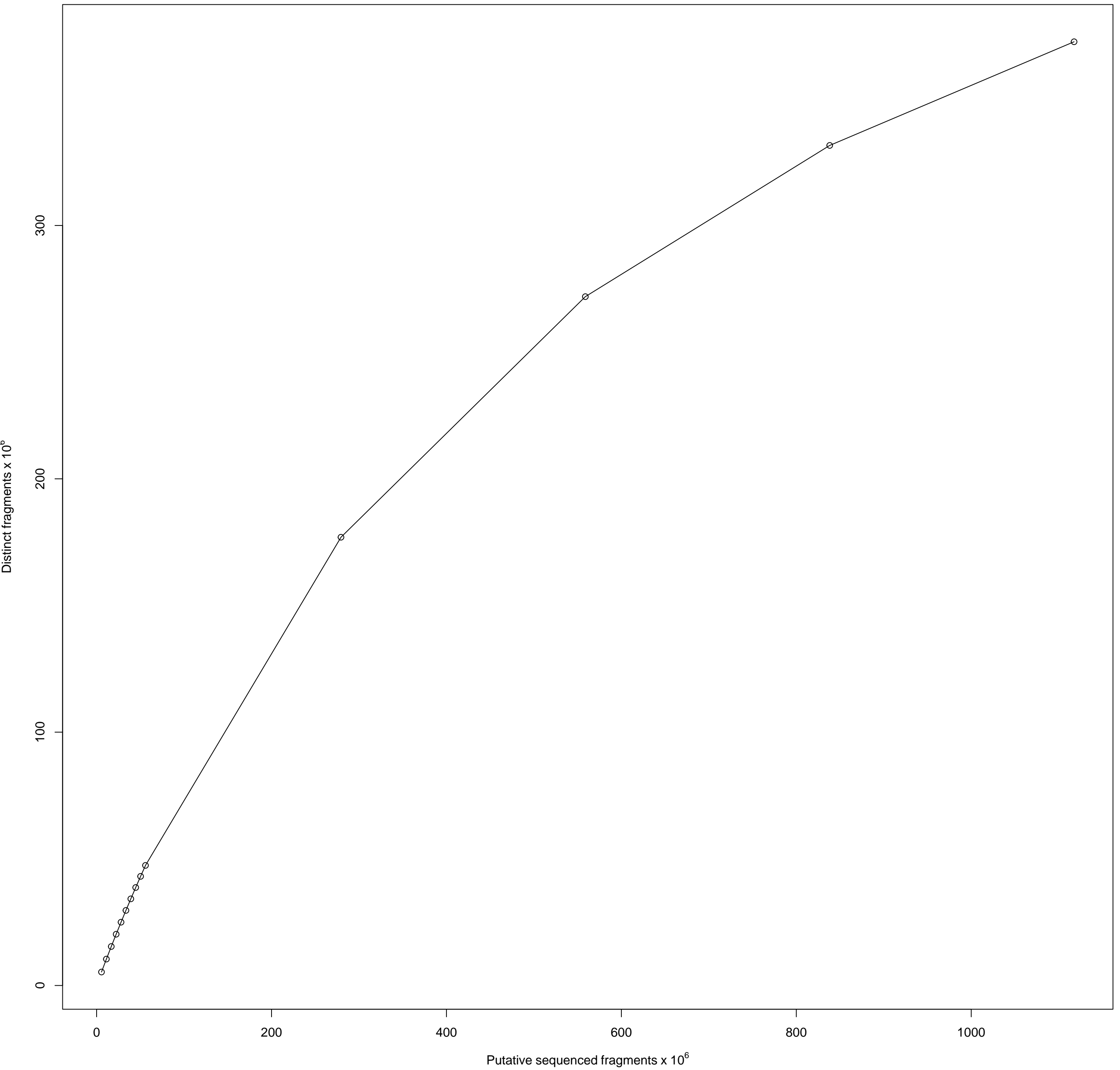
Estimation of ATAC-seq library complexity
