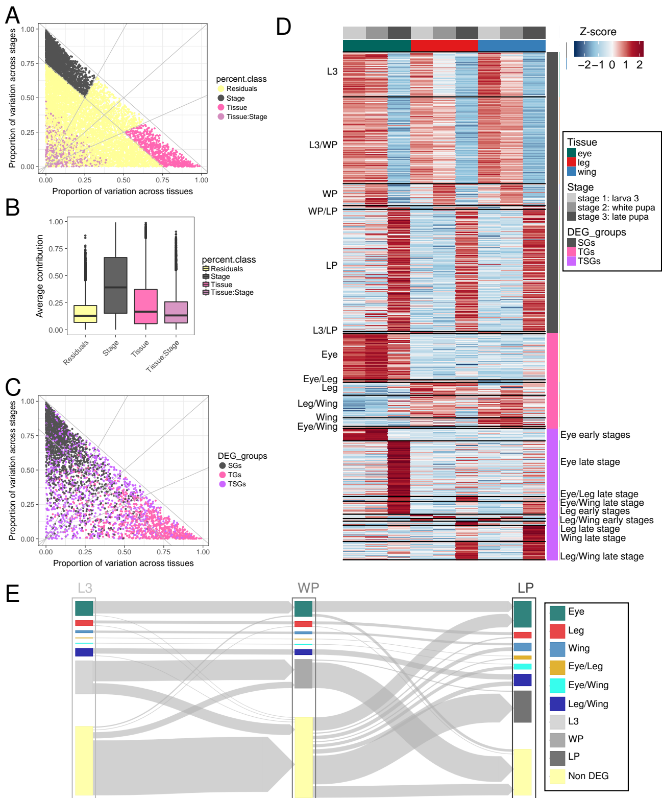
Fig. 2 RNA dynamics through tissues along fly development. (a) Proportion of the gene expression variation explained by tissues ( x -axis) and by developmental stages ( y -axis) for 9334 genes ( dots ; i.e. genes expressed at least 5 TPMs in two samples) using linear models. The gray lines at y = 2x and x = 2y identify the genes in which tissue-explained variability is two fold greater than developmental stage-explained variability, and in which developmental stage-explained variability is two fold greater than tissue-explained variability, respectively. We restricted to the genes for which either tissue or stage explains at least 75% of the variability ( gray line at x + y = 0.75 ). We defined 4 sets of genes: (i) genes whose expression varies considerably across stages and little across tissues, SGs ( gray ); (ii) genes whose expression varies considerably across tissues and little across stages, TGs ( pink ); (iii) genes whose expression varies considerably across tissues as well as across stages, TSGs ( purple ); and (iv) genes with variation due to interaction tissues:stages, iTSGs ( dark pink ). (b) Box plot representing the distribution of the proportion of gene expression variation across stages and tissues, where stages show higher contribution to gene expression variability than tissue or the interaction tissue:stage. (c) Differentially expressed genes (DEG) across tissues (TGs), stages (SGs) and both tissue and stage (TSGs) were defined using edgeR (Robinson et al., 2010). They are 793, 2340 and 1097 genes, respectively. The proportion of the gene expression variation explained by tissues ( x -axis) and by developmental stages ( y -axis) of those genes ( dots ) are shown. As expected such genes are concordant with the higher gene expression variability in tissues or developmental stages. (d) Heatmap of DEG across tissues (TGs), stages (SGs) and both tissue and stage (TSGs). Gene expression values are normalized to z -scores. There are more stage-specific genes than tissue-specific genes. Genes were further classified in subgroups based on upregulation in precise tissues/stages. (e) Dynamics of DEG across fly development. Notably there are more eye, leg and wing-specific genes, respectively, at the late stage.
