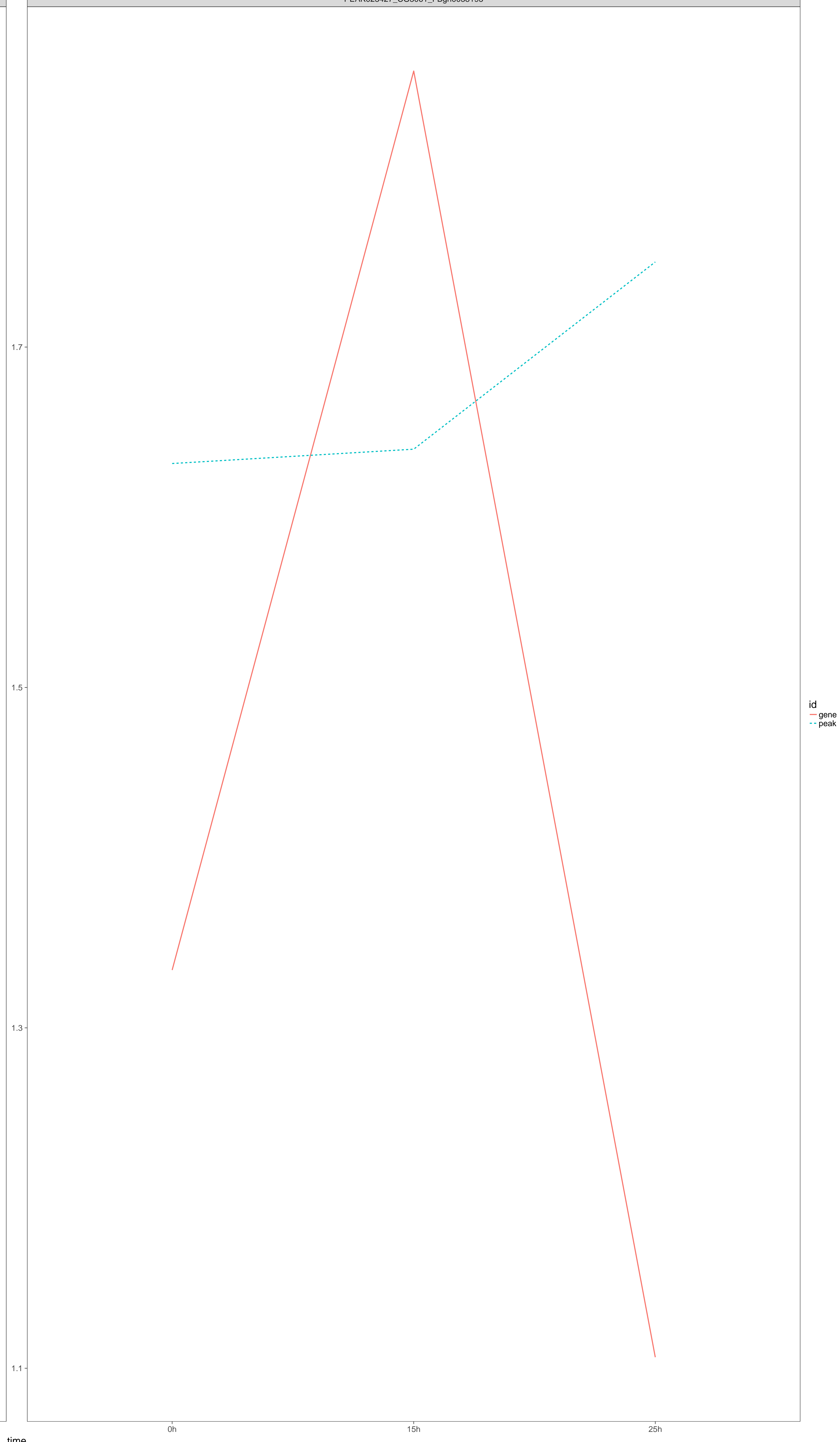
PEAK023427_CG3061_FBgn0038195
