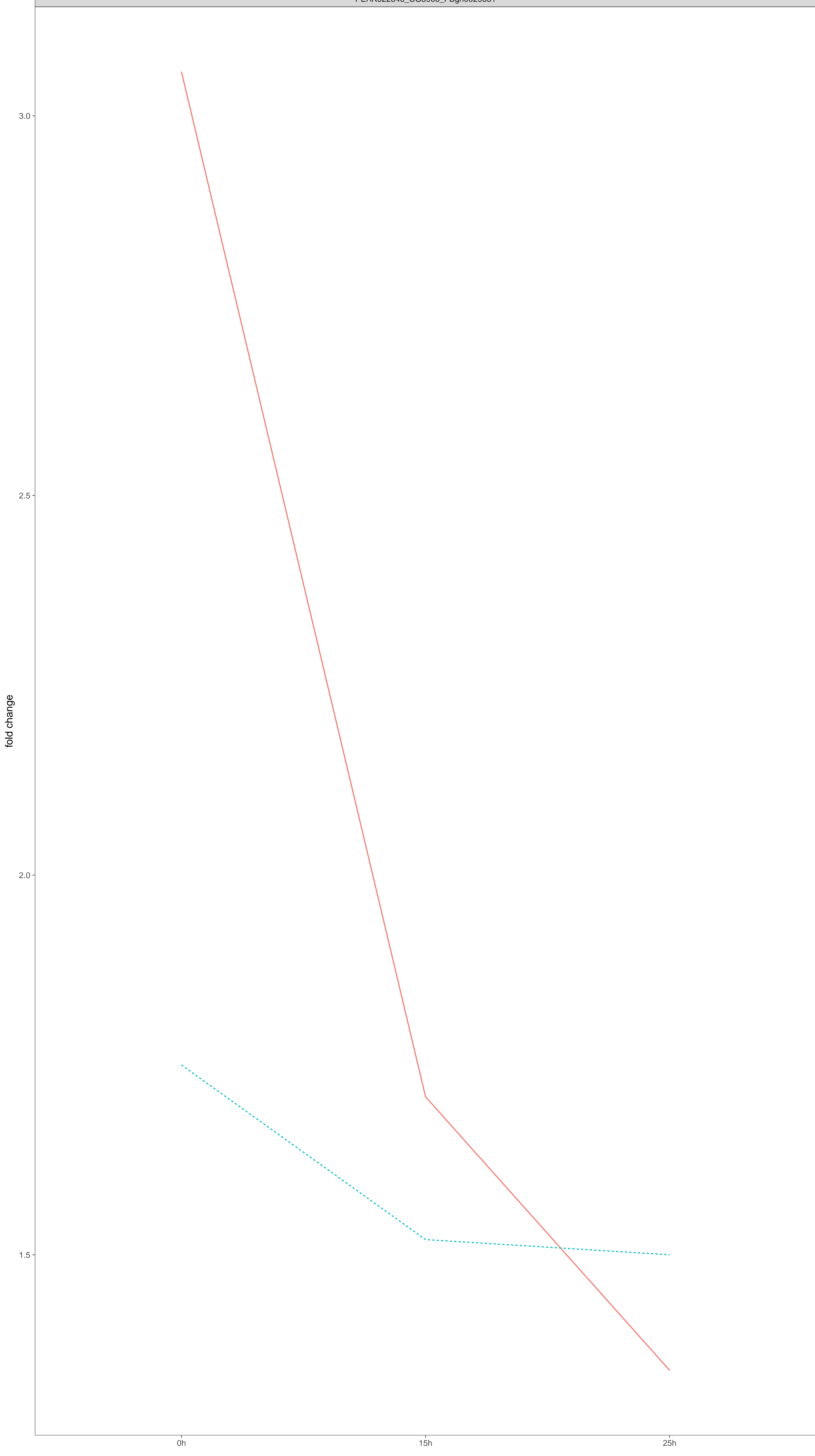
PEAK022846_CG5966_FBgn0029831
