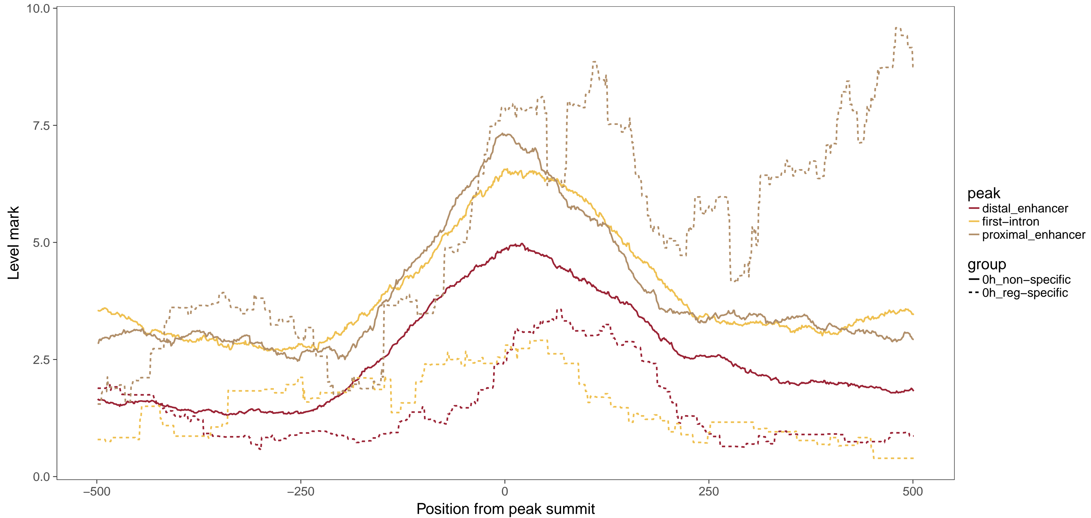
chip_BEAF-32_WID_Rep2_Gurudatta-et-al-2012_SRR447743
