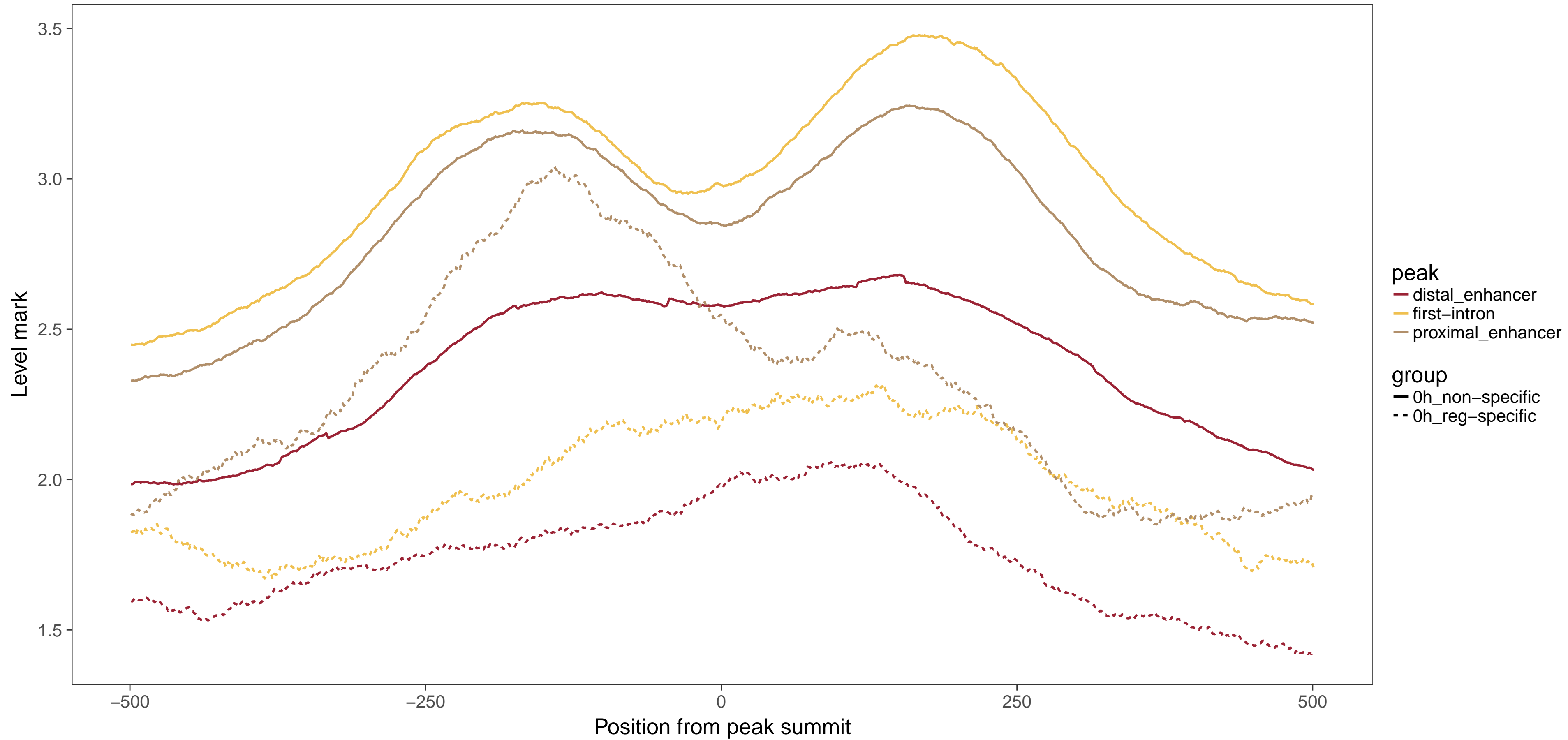
chip_ASH2_WID_Rep1_Perez-et-al-2011_SRR065624
