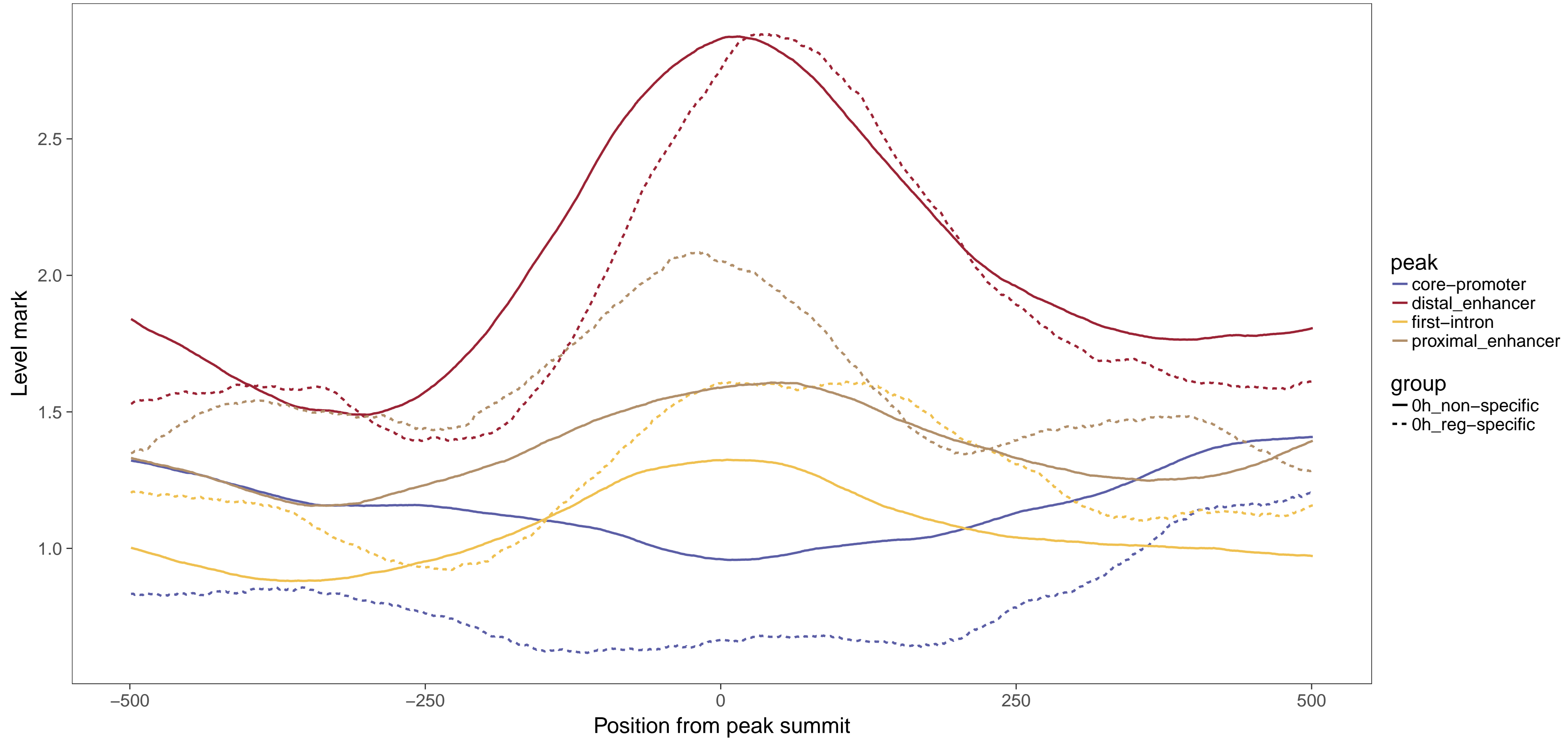
chip_K27me3_WID_Rep1_Cavalli-et-al-2016_SRR2672985
