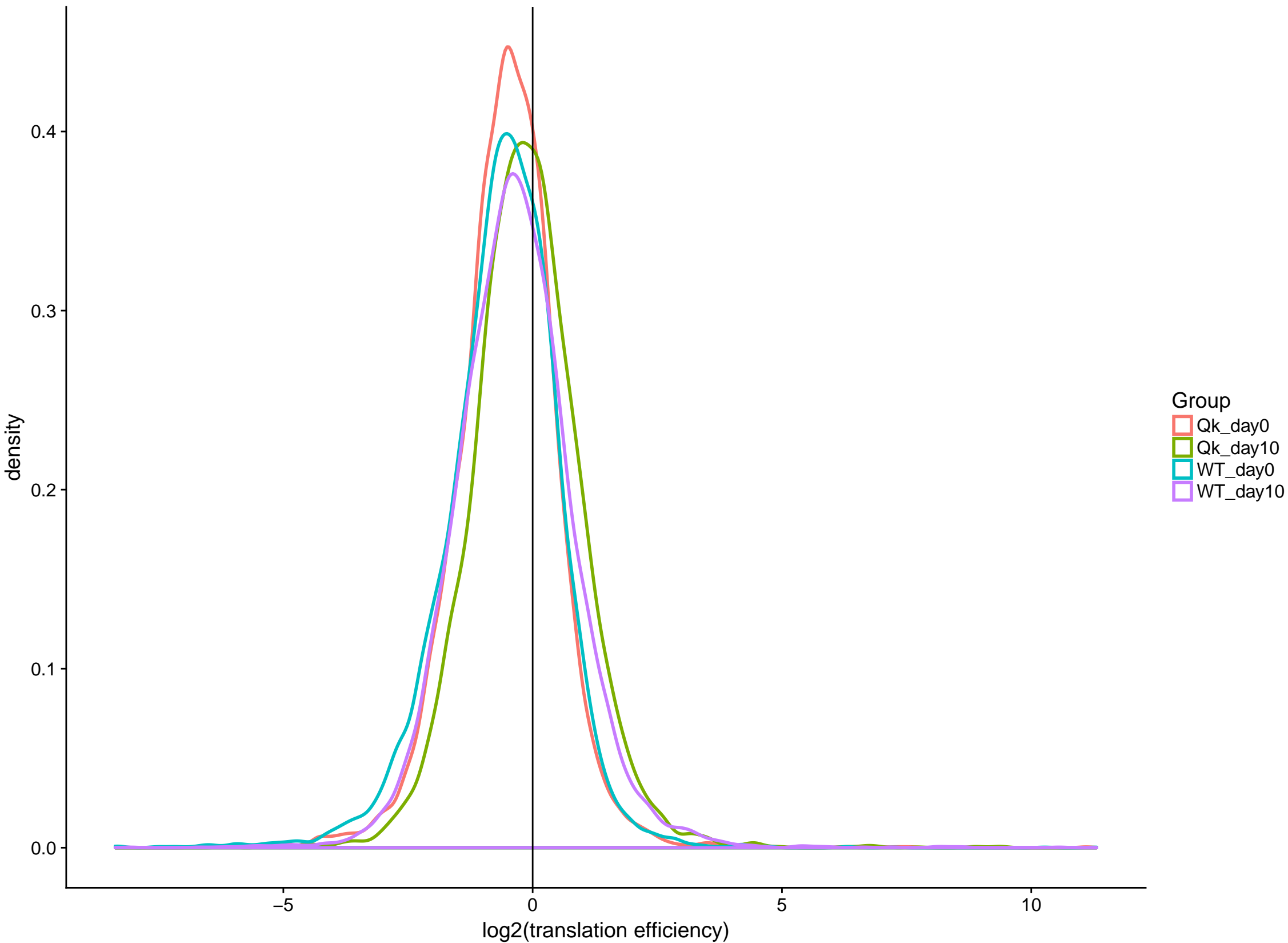
Translation efficiency calculated per experimental group
