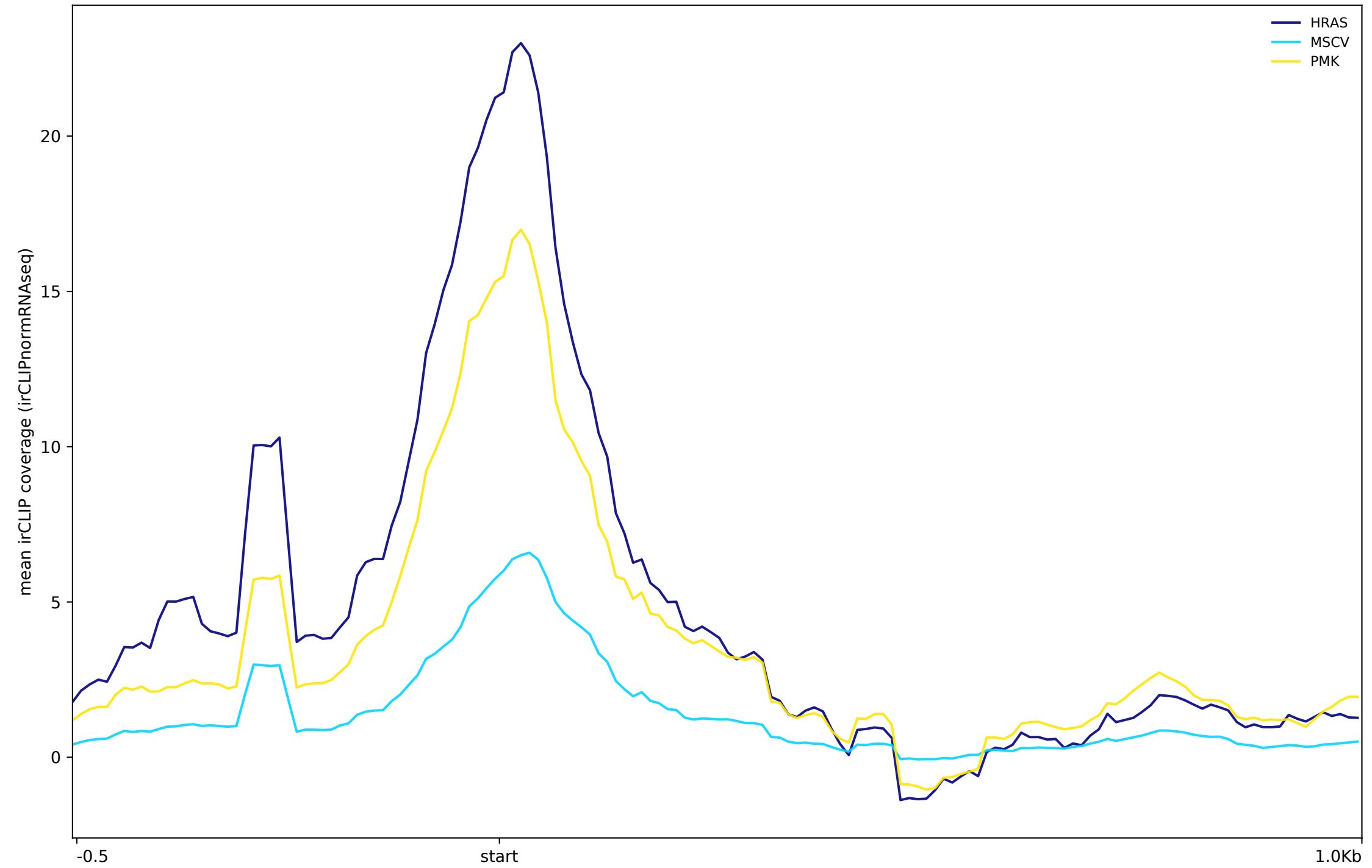
Coverage of irCLIPnormRNAseq signal around genes deseq2diffbind pvalue005 nohigh start codon
