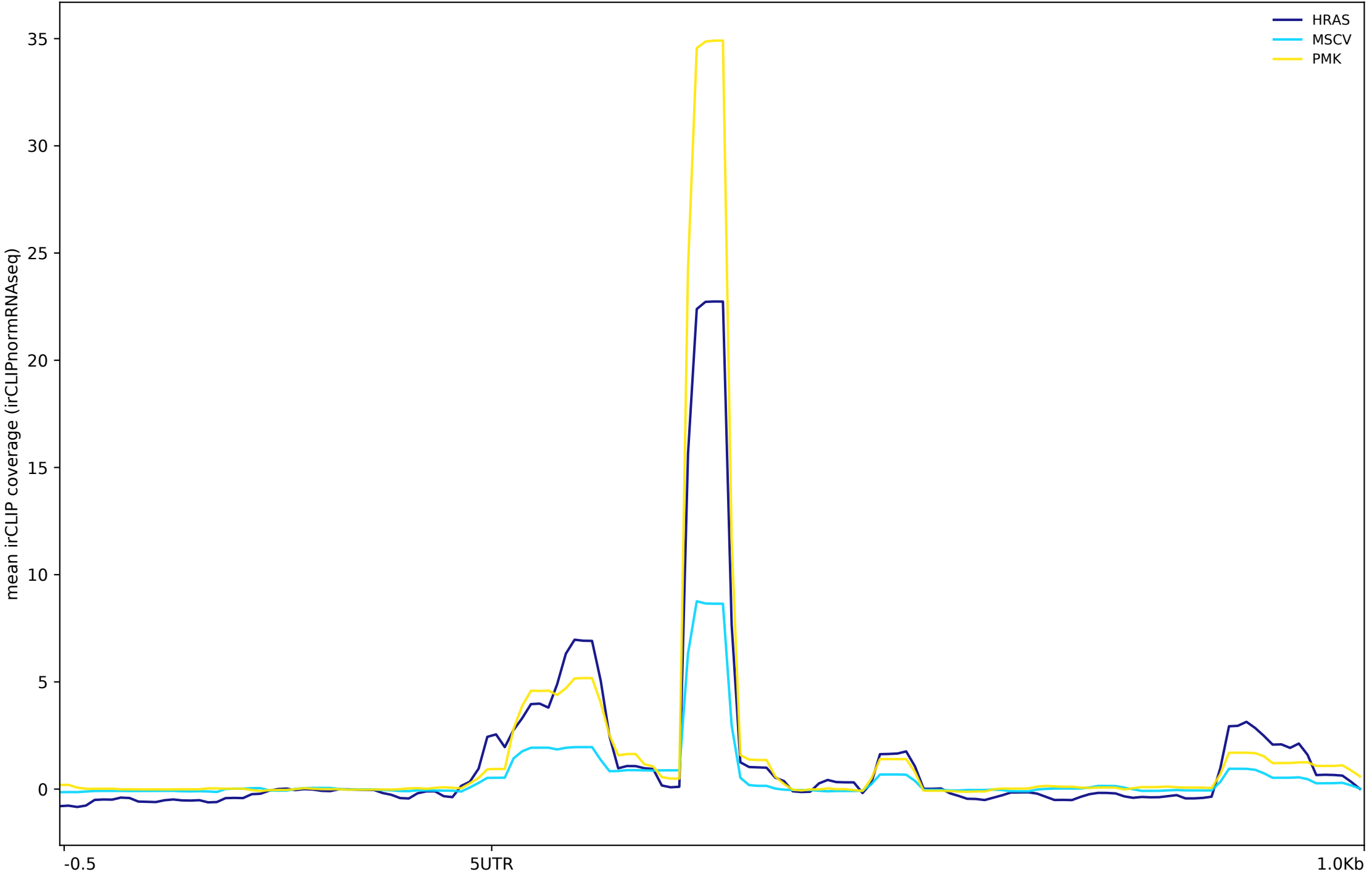
Coverage of irCLIPnormRNAseq signal around genes 1000random 5utr
