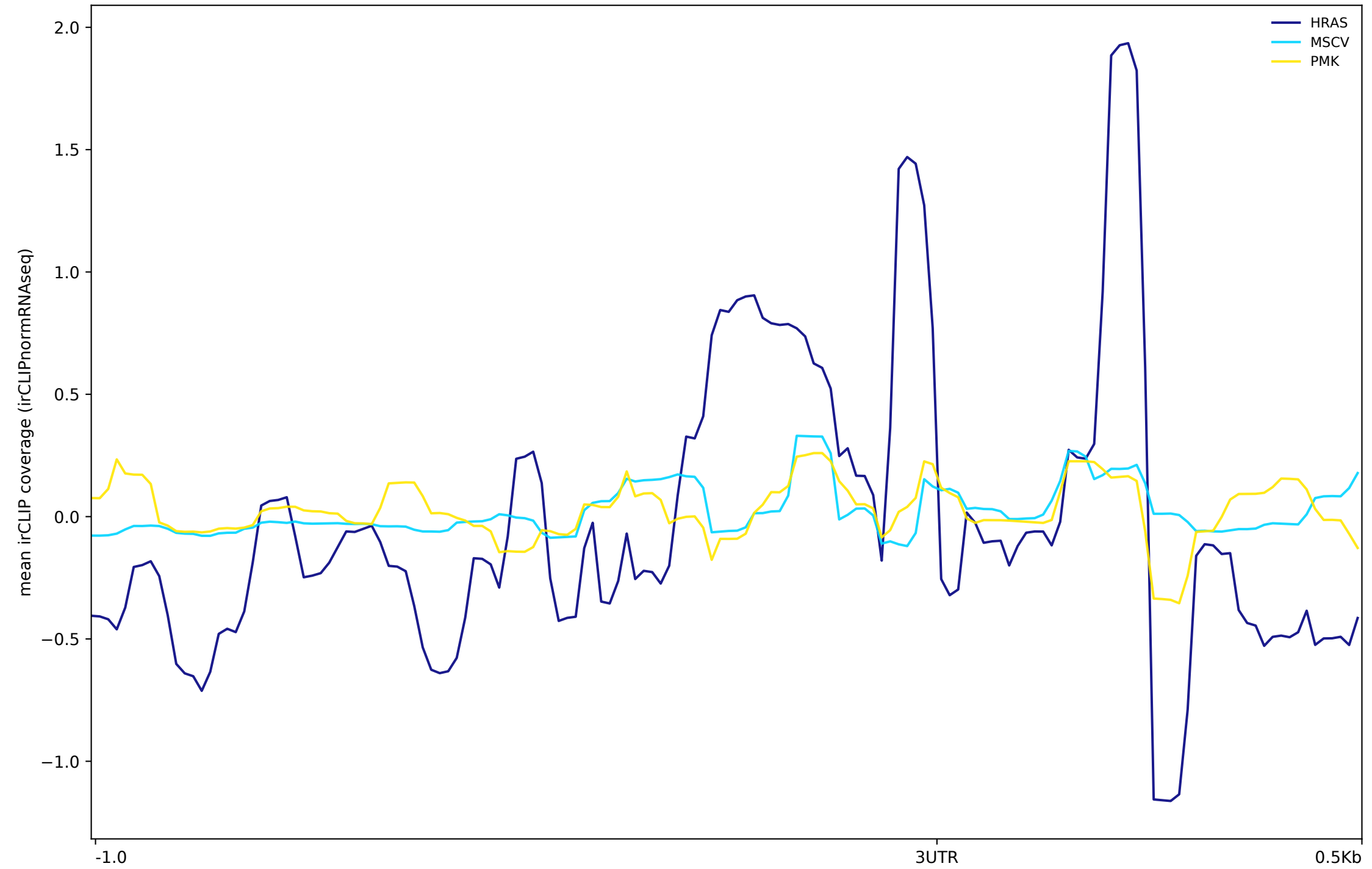
Coverage of irCLIPnormRNAseq signal around genes 1000random 3utr
