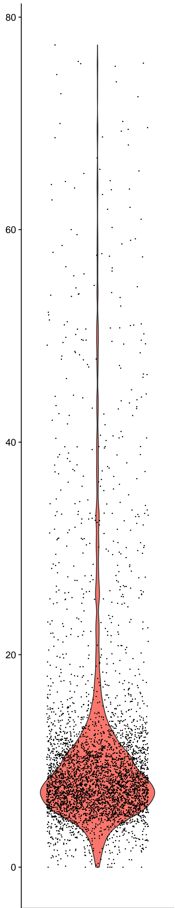
percent.mt
