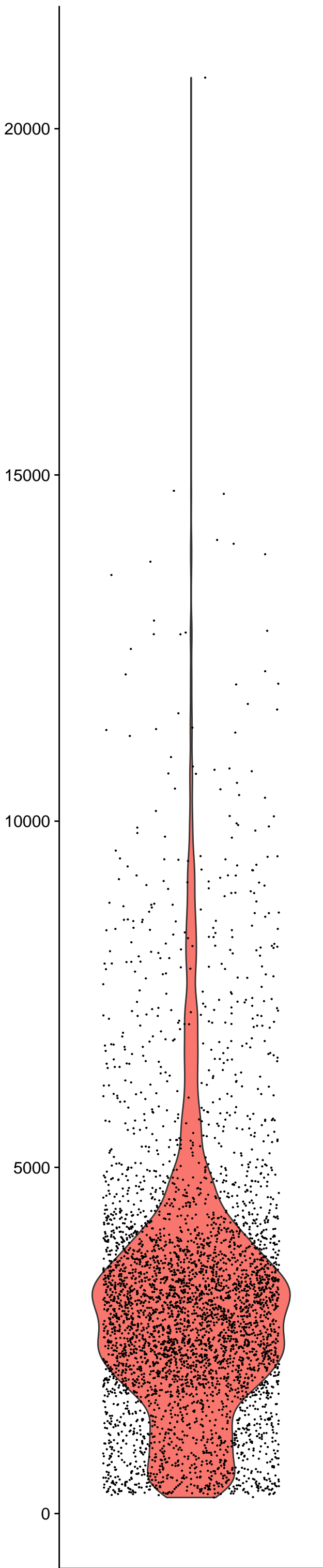
nCount_RNA
