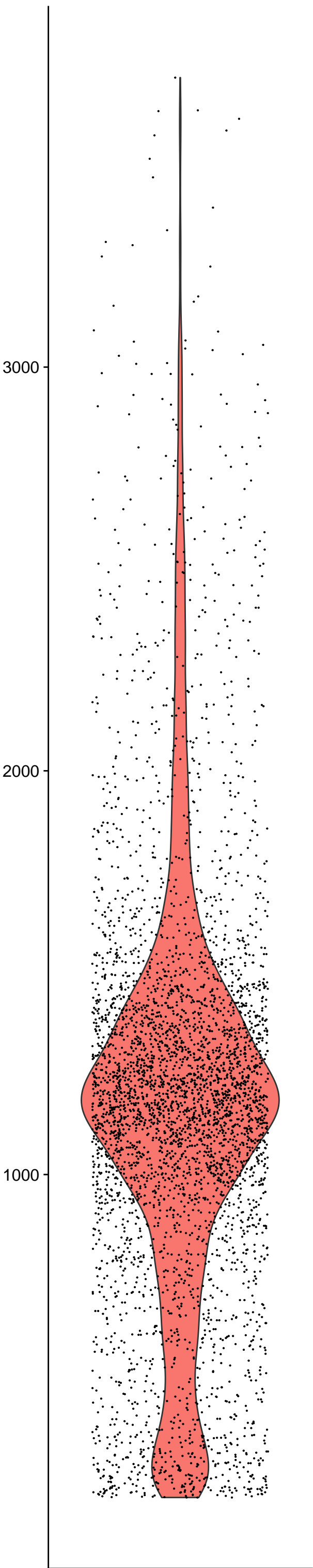
nFeature_RNA
