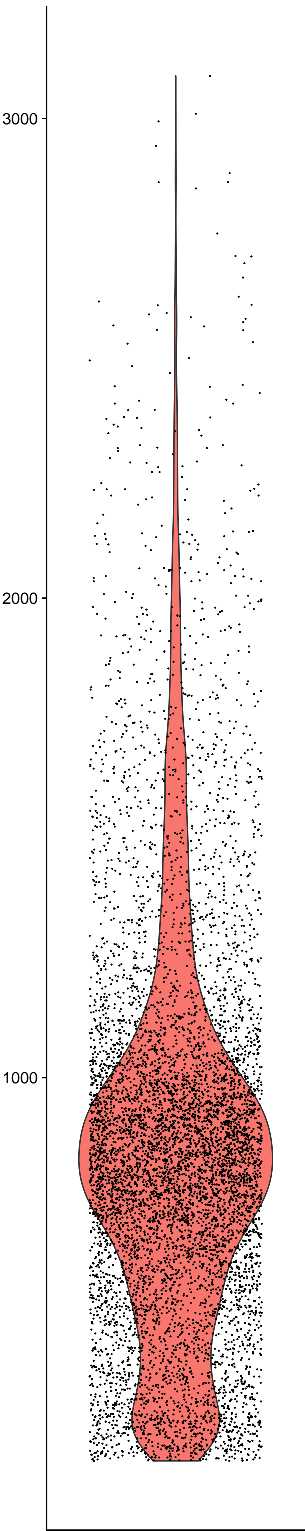
nFeature_RNA
