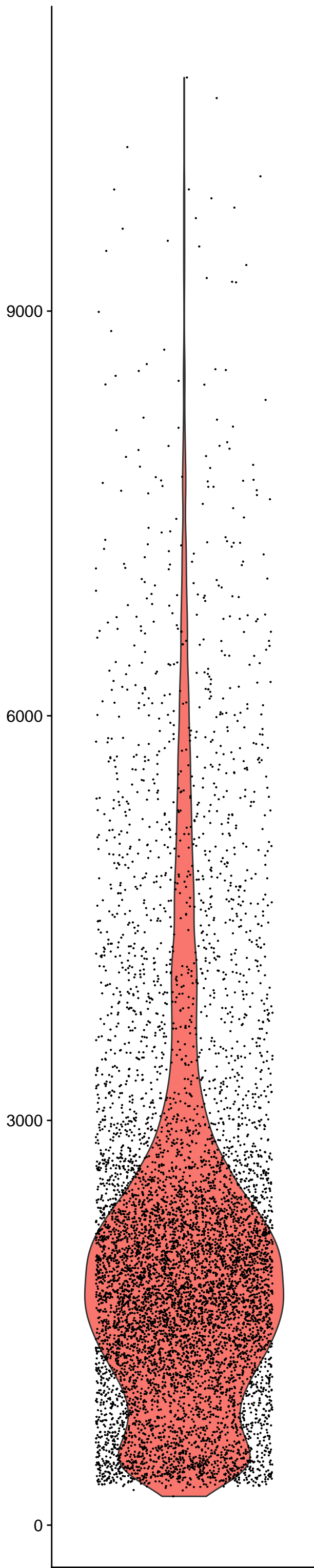
nCount_RNA
