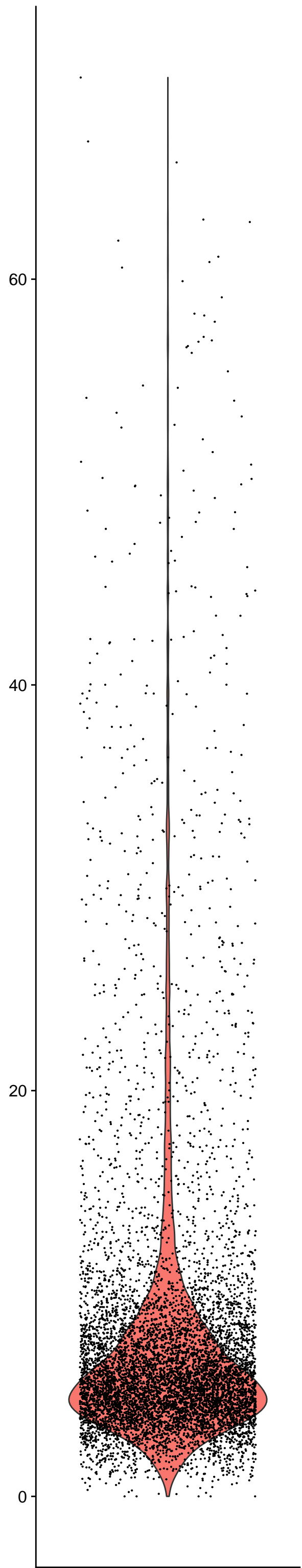
percent.mt
