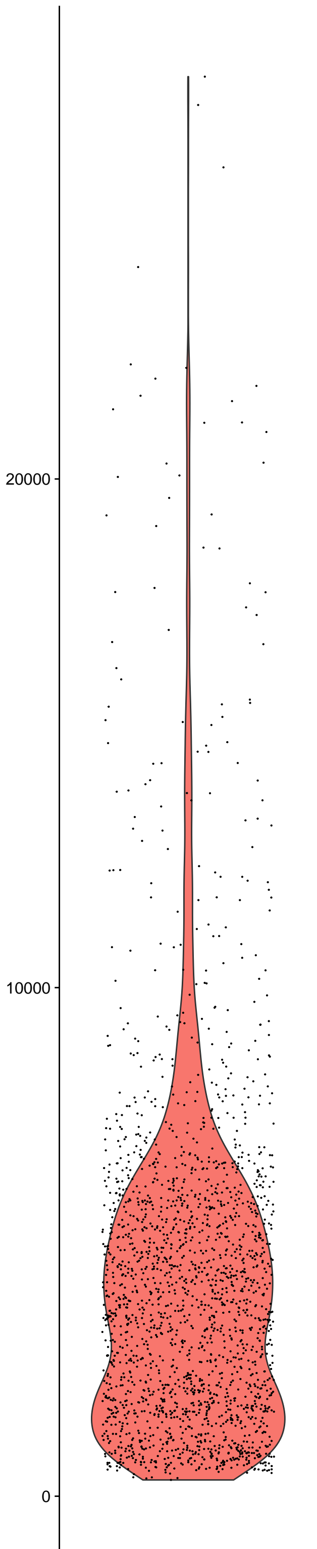
nCount_RNA
