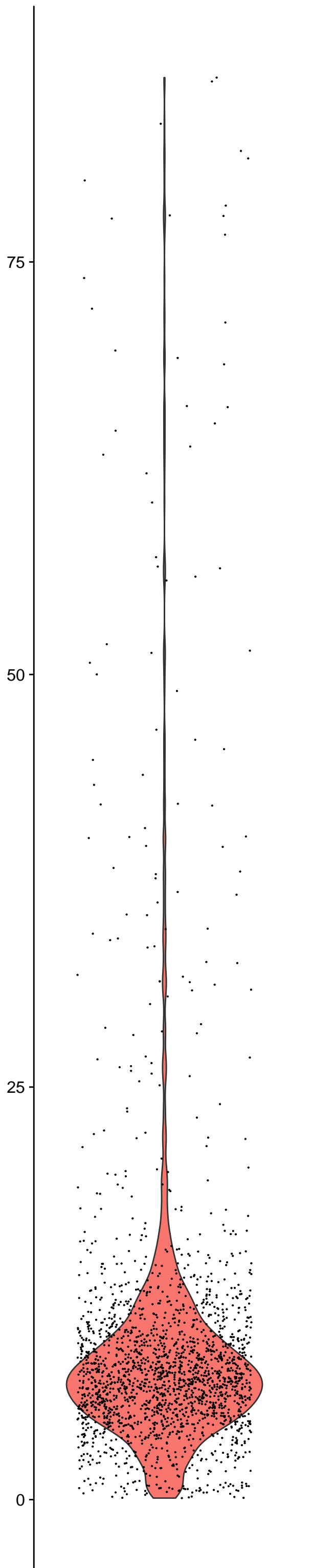
percent.mt
