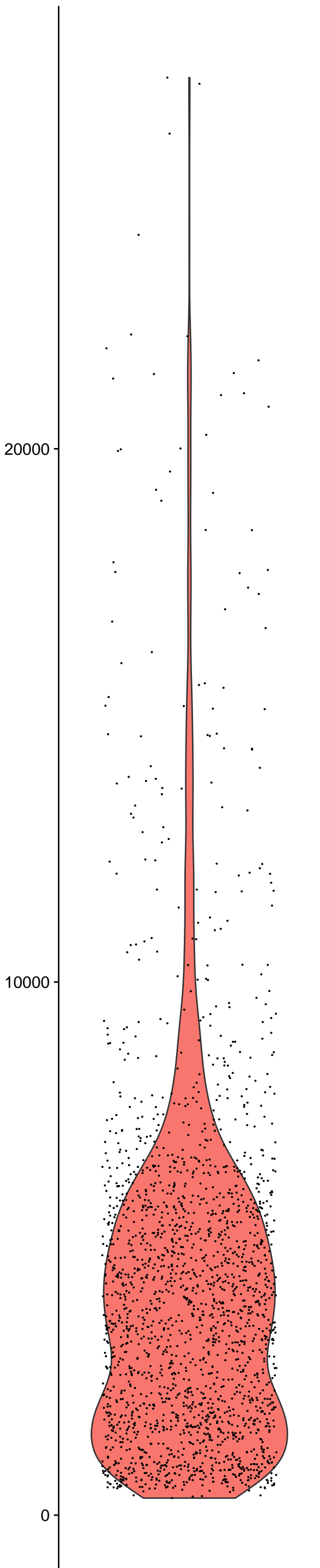
nCount_RNA
