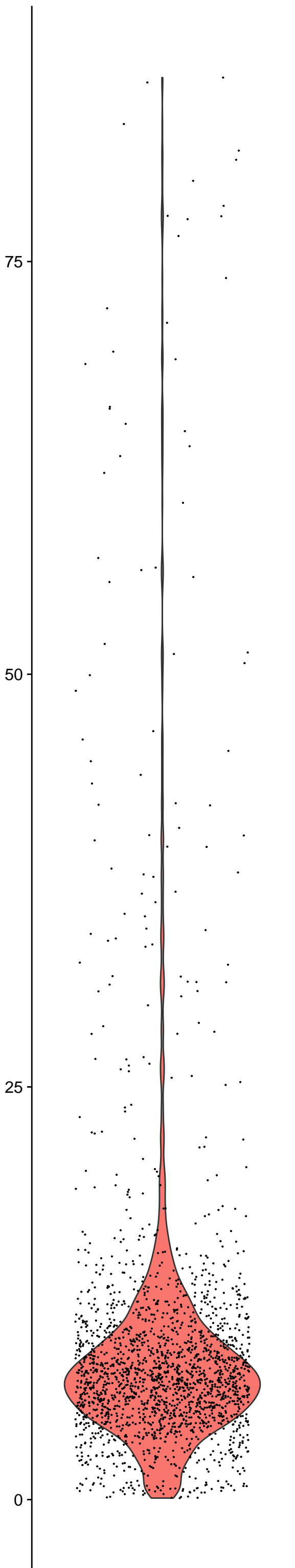
percent.mt
