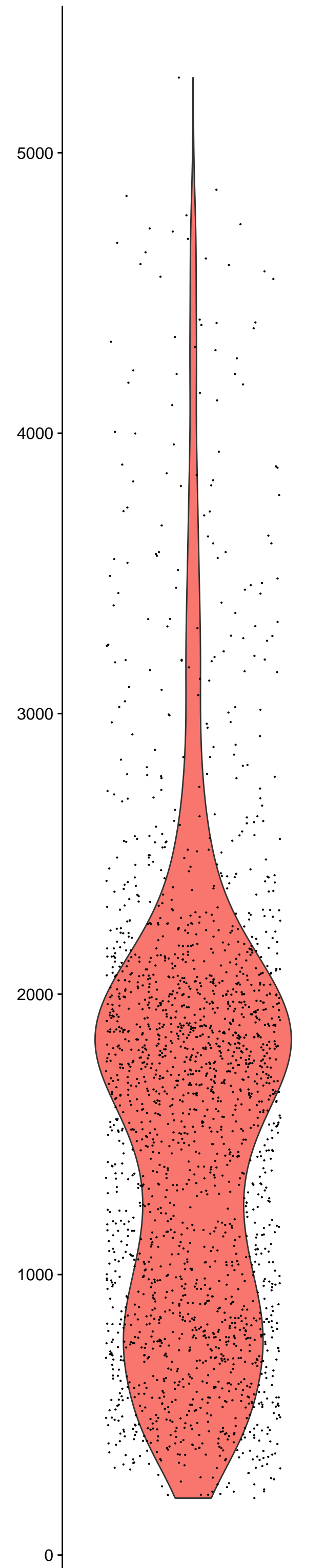
nFeature_RNA
