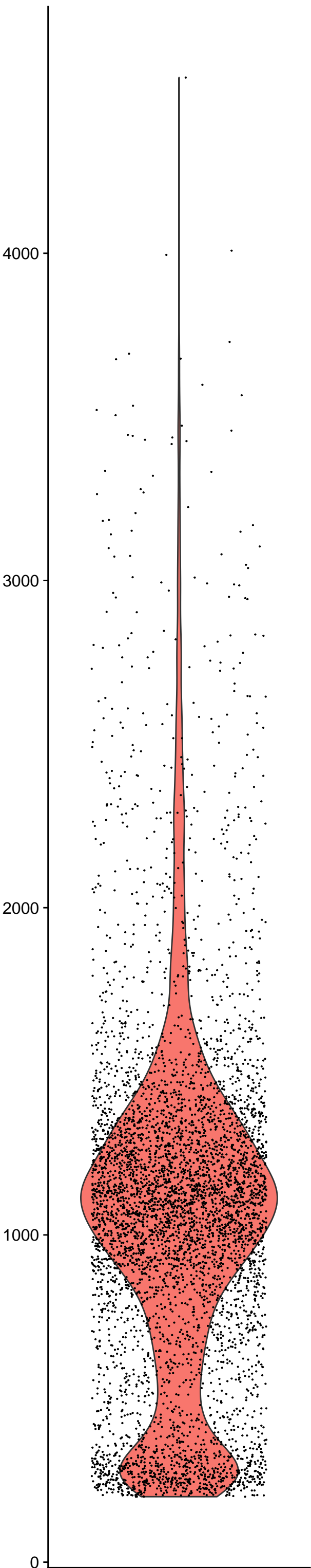
nFeature_RNA
