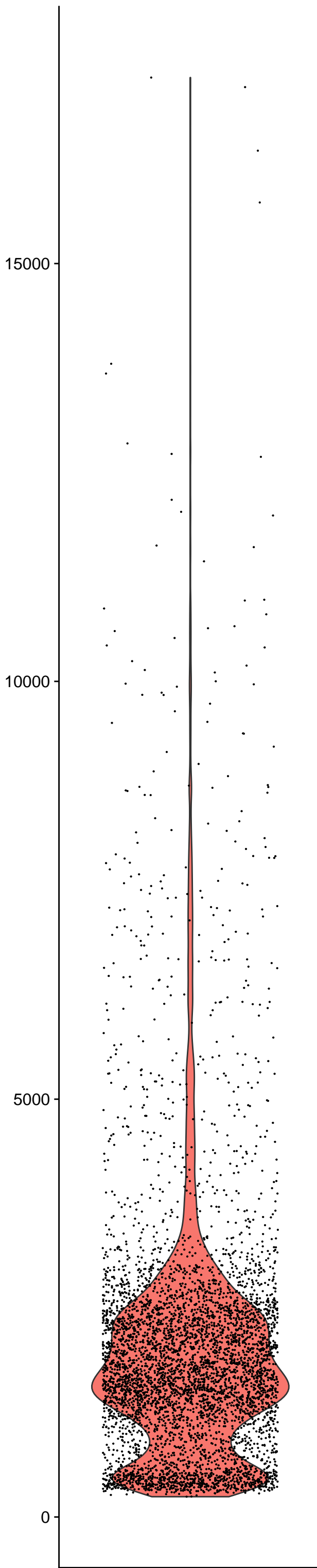
nCount_RNA
