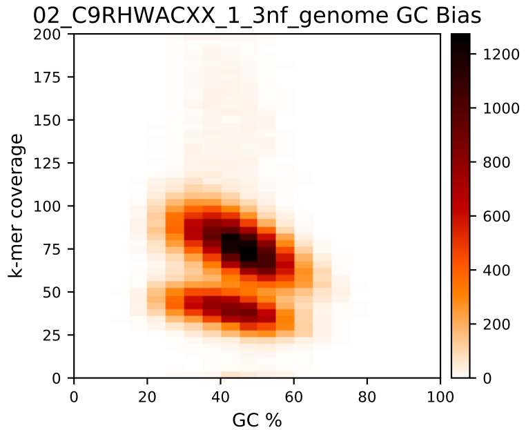
bird GC Bias
